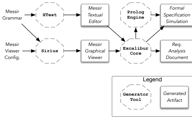
Figure 1. Excalibur workbench architecture
