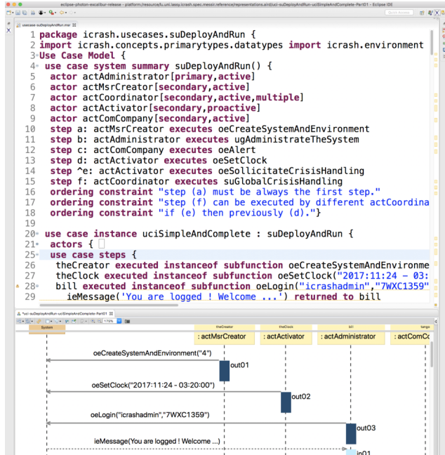
Figure 2. An Excalibur screenshot with use-case textual specifications and a use-case instance graphical view
