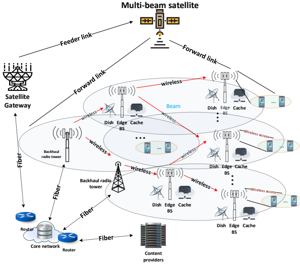
Fig. 2: Hybrid satellite-terrestrial network using a multi-beam satellite for more accurate content placement phase.
