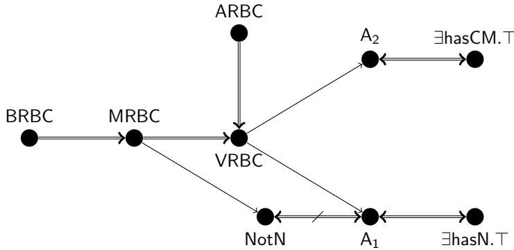
Figure 1: Inheritance net built from Example 10.
