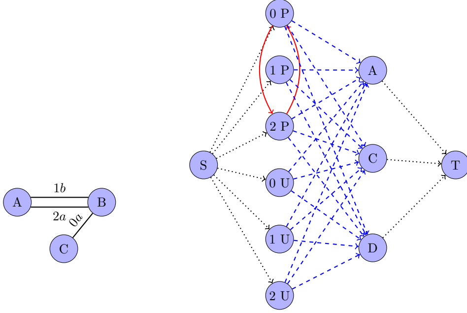
Figure 2: Left a line planning possibility and right the resulting flow graph ( G_F = (N_F, A_F) ). The arcs from and to the source and sink are dotted black, the interchange arcs ( A_I^d ) solid red and the arcs to the facilities ( A_C ) are dashed blue.
