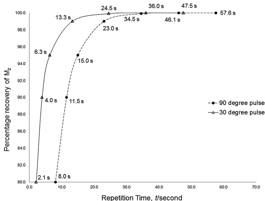
Fig. 1 Relationship between targeted accuracy and the minimum required repetition time, t . Triangles and circles correspond to experiments with 30^\circ and 90^\circ pulse angle, respectively. The longest T_1 of carbonyl carbons is set at 5.0 seconds.
