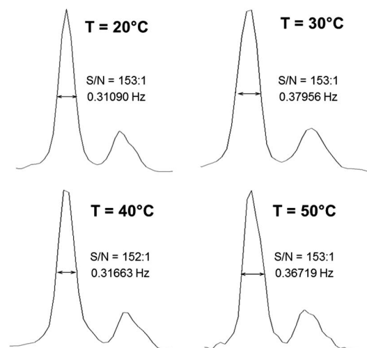
Fig. 2 Effect of experimental temperature ( T = 20^\circ\text{C} , 30^\circ\text{C} , 40^\circ\text{C} and 50^\circ\text{C} ) on peak width and S/N ratio of cis -9 monoene acyl chain carbonyl resonances of triacylglycerols in rapeseed oil (canola). Temperature control was used to maintain constant temperature throughout the experiment.
