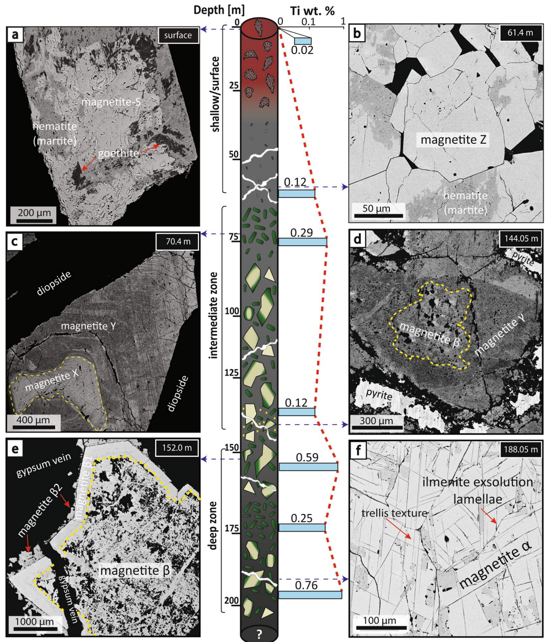
Figure 2. Schematic illustration of a representative drill core from Laco Norte (LCN-0944) showing the morphology and lithological variations of the ore bodies. The dashed red line and light blue bars indicate the average Ti concentration of the magnetite from the surface to the base of the drill core. Backscattered electron (BSE) images show the different textural types of magnetite. (a) Euhedral, altered and porous Magnetite-S grain from a surface sample showing pervasive replacement by hematite and goethite along grain boundaries, fractures, and pores. (b) Aggregate of pristine Magnetite-Z grains, weakly oxidized to hematite (sample depth 61 m). (c) Microcrystalline core of pristine Magnetite-X showing evidence of dissolution-reprecipitation processes. Magnetite-Y overgrowths Magnetite-X, and exhibits alternating bands of Ti-bearing inclusions, which are responsible for the increase in the magnetite Ti concentration within this zone (sample depth 70.4 m). (d) Ti-poor Magnetite- \gamma from pyrite-rich massive magnetite zone associated with gypsum veinlets. Magnetite- \gamma overgrowth developed on an inclusion-rich Magnetite- \beta core and displays sector zoning with inclusion-rich areas (sample depth 144 m). (e) Euhedral core of inclusion-rich Magnetite- \beta surrounded by a pristine inclusion-free-rim of Magnetite- \beta_1 . Both magnetite types have high Ti contents. Irregular grains of Ti-poor Magnetite- \beta_2 associated with late crosscutting gypsum veinlets developed over Magnetite- \beta_1 rims (sample depth: 152 m). (f) Aggregate of Ti-rich Magnetite- \alpha grains showing well-developed ilmenite exsolution lamellae, which exhibit both trellis and sandwich textures (sample depth 188.05 m).
