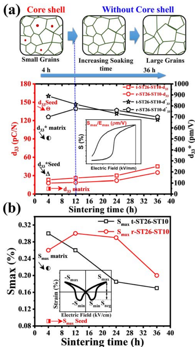
Figure 7. (a,b) Piezoelectric constant d_{33} , normalized strain d_{33}^* , and maximum bipolar strain ( S_{\text{max}} ) as a function of different soaking times of the composites. Contribution of the core of a ferroelectric seed in a matrix is analyzed for the evolution of polarization, strain and phase transition.
