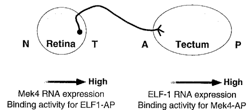
Figure 7. Complementary Expression and Binding of ELF-1 and Mek4 in Relation to Retinotectal Topographic Mapping
