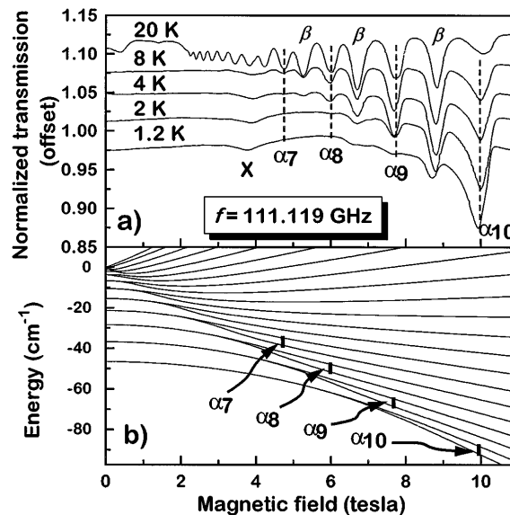
FIG. 3. (a) EPR spectra obtained at several temperatures, for \mathbf{B}_0 \perp \mathbf{c} (see text for explanation of labels). (b) A calculation of the corresponding energy levels [13]; the arrows indicate the transitions responsible for the resonances in (a).
