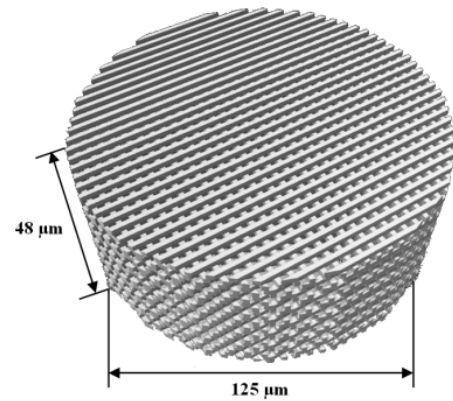
(a) Design of 3D PhC woodpile structure of a cylinder shape.
