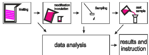
Fig. 3. The block diagram of the experiment
