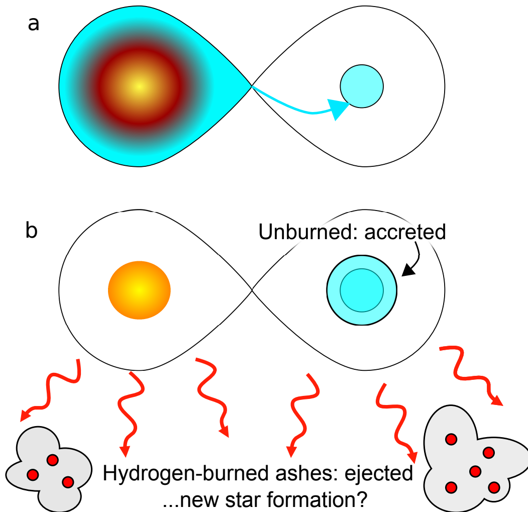
Figure 1. Schematic view of Roche-lobe overflow in a massive binary system. (a) At the start of Roche-lobe overflow, the primary star (left) overflows its Roche lobe and transfers material to the secondary (right). (b) By the end of Roche-lobe overflow, the secondary has accreted unburned material while hydrogen-burned material from deep inside the primary has been ejected from the binary system and may mix with other sources of interstellar gas from which a subsequent generation of stars may form.
