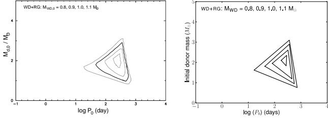
Fig. 5. Initial parameter regions for the WD+RG track to SNeIa. The different contours are for different WD masses (increasing in size with increasing mass) and the stripping parameter c_1 = 1 . Left: from HKN99b. Right: initial parameter regions as used in this work.
