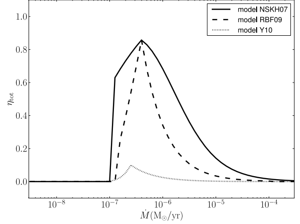
Fig. 3. Total retention efficiencies, resulting from different combinations of the hydrogen and helium retention efficiencies. In this figure we have assumed M_{\text{WD}} = 1 M_{\odot} as an example. The mass transfer rate \dot{M} = |\dot{M}_{\text{comp}}| . For lower (higher) M_{\text{WD}} the maximum retention efficiency shifts to lower (higher) |\dot{M}_{\text{comp}}| . For a more detailed explanation of the retention efficiencies see Sect. 3.1.
