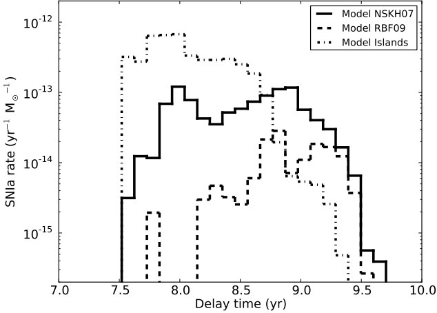
Fig. 7. Same as in Fig. 6 but assuming the \alpha -formalism with \alpha\lambda = 0.5 . Again no SD binaries evolve into a SNeIa for the retention efficiency of Y10.
