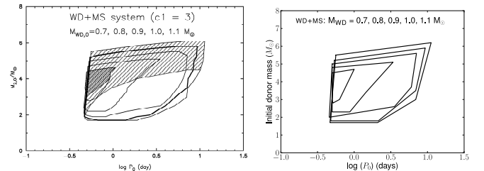
Fig. 4. Initial parameter regions for the WD+MS track to SNIa. The different contours are for different WD masses (increasing in size with increasing mass) and the stripping parameter c_1 = 3 . Left: from HKN08. The hatched regions indicate SNIa explosions with short delay times of t < 100 \text{ Myr} for M = 0.7 M_{\odot} and M = 1.1 M_{\odot} . Right: initial parameter regions as used in this work.
