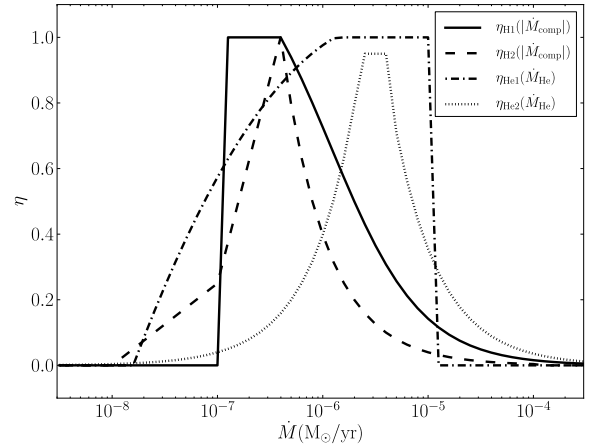
Fig. 2. Examples of hydrogen and helium retention efficiencies as a function of the mass transfer rate for a WD of 1 M_\odot . The prescriptions for the hydrogen retention efficiency \eta_{H1} (solid line - NSKH07; HKN08) & \eta_{H2} (dashed line - RBF09; Y10) and the helium retention efficiency \eta_{He1} (dot-dashed line - Hachisu et al. 1999a; Kato & Hachisu 1999) & \eta_{He2} (dotted line - Iben & Tutukov 1996) are shown in Appendix A. Note that the position of the peak of \eta_{H2} is dependent on the exact prescription for \dot{M}_{cr} . The mass transfer rate for hydrogen accretion is given by |\dot{M}_{comp}| . For helium accretion this is \dot{M}_{He} .
