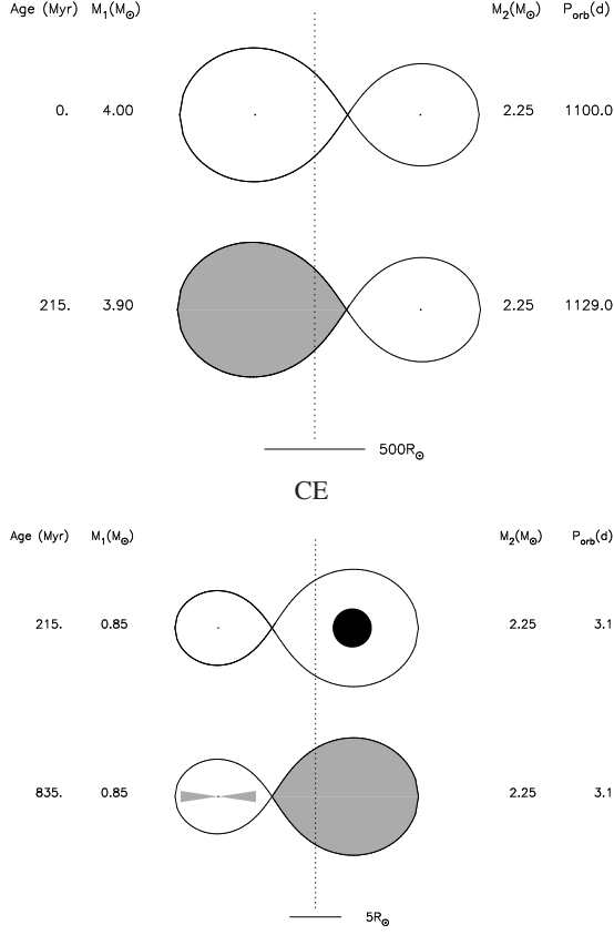
Fig. 1. Binary evolution for a single-degenerate SNIa progenitor. In this case the donor is a MS star. The top and bottom parts of the figure have different scales due to the common envelope phase, denoted as CE in the figure.
