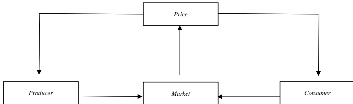
Fig. 1. Free market system (Šnapka and Dvořáček, 1995).
