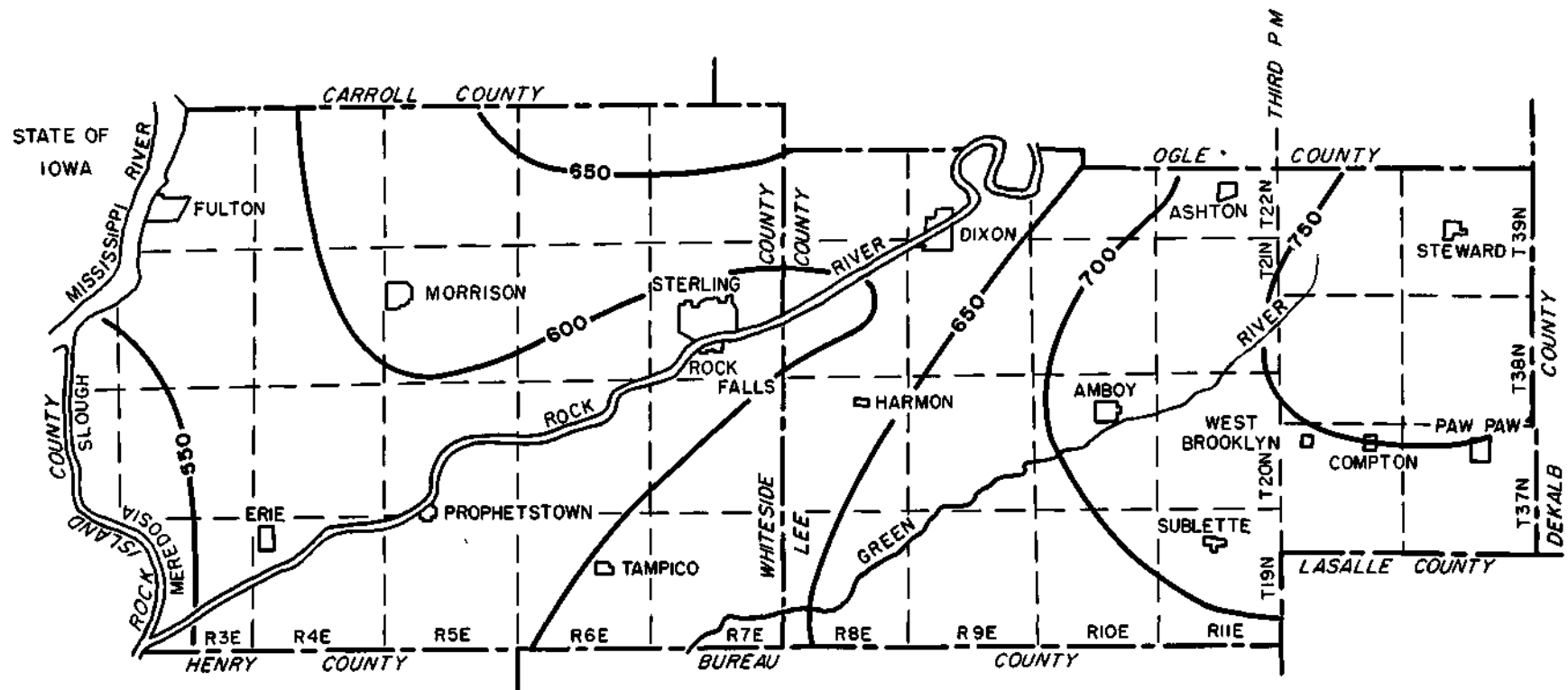
FIG. 4 - WATER SURFACE CONTOURS FOR SANDSTONE
