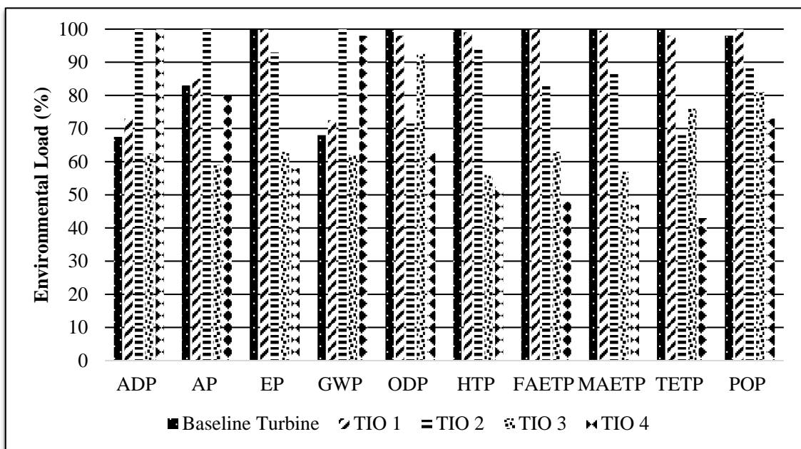
Figure 3. Characterization results for the comparison between the construction stages of the baseline turbine and TIOs 1
