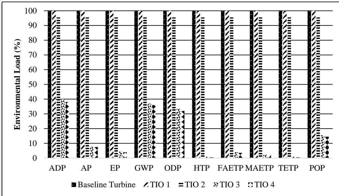
Figure 4. Characterization results for the comparison between the operation stages of the baseline turbine and TIOs 1 - 4
