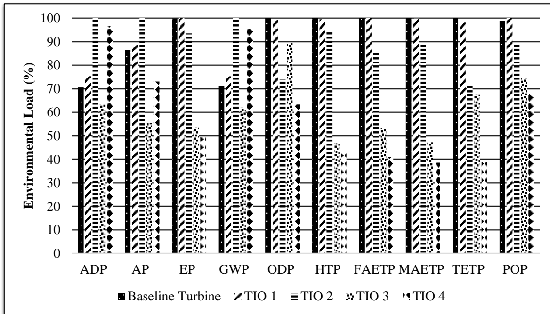
Figure 2. Characterization results for life cycle environmental impacts of the wind farm for the baseline turbine compared to TIOs 1 – 4
