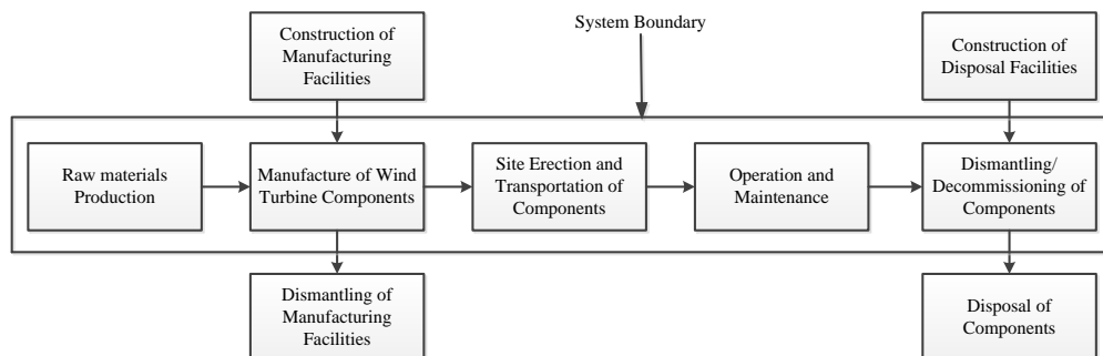
Figure 1. Boundary for the life cycle of the wind farm
