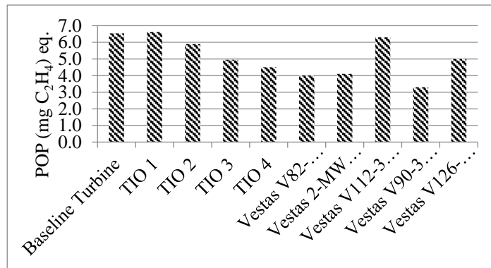
Figure 6. Estimated GWP, AP and POP for the wind farm using the different design variations compared with literature
