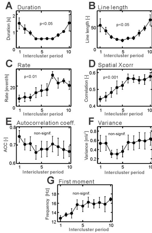
Figure 7 Changes in the properties of epileptic bursts between clusters of seizures. (a) With the approaching cluster the duration of the bursts increase, as well as, the line length parameter (b) . (c) The proximity to critical transition is also marked by the increasing rate of epileptic bursts. (d) Increase in spatial correlation reflects enhanced propagation of bursts to the hippocampus and motor cortex. (e) The autocorrelation, signal variance (f) and the first spectral moment (g) did not show significant changes with approaching cluster. The significance of changes in temporal profiles was analyzed using one-way ANOVA. Error bars, s.e.m.
