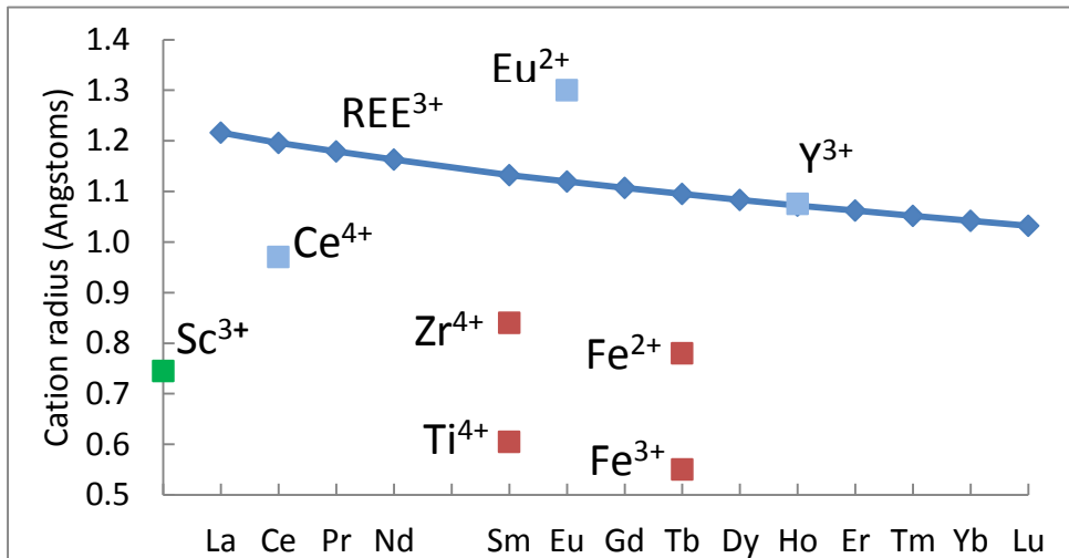
Figure 1 The lanthanide contraction - smooth variation in cation radii of the +3 REE cations, La through to Lu and Y, compared with the larger and smaller \text{Eu}^{2+} and \text{Ce}^{4+} cations and the much smaller \text{Sc}^{3+} cation is key to understanding REE distribution in minerals. Sc is more likely to substitute into minerals containing Zr, Ti, Fe than to partition with the other REE. Zr, Ti and Fe are plotted at arbitrary positions on the x axis. Graph from Siegfried et al. (2018).
