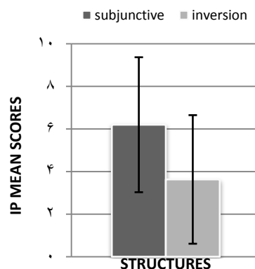
Figure 2. Trend of Development (Subjunctive vs. Inversion)
