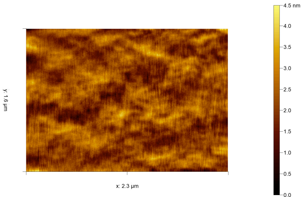
Figure 4. Selected contact mode HS-AFM frame of Emiliana huxleyi cell surface captured at 0.5 s per frame by the authors. Variations in height are likely due to membrane ruffles, localised variation in membrane lipid composition/size and their associated membrane proteins.
