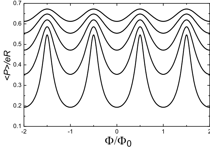
Fig. 7 Magneto-oscillations of the dipole moment of a ring at various magnitudes of the in-plane electric field for T = 0.01\varepsilon_1(0)/k_B . Different curves correspond to different magnitudes of the electric field in the range from E = 0.2\varepsilon_1(0)/eR to E = 1.0\varepsilon_1(0)/eR with the increment 0.2\varepsilon_1(0)/eR . The upper curve corresponds to E = 1.0\varepsilon_1(0)/eR . (From Ref. [3]).
