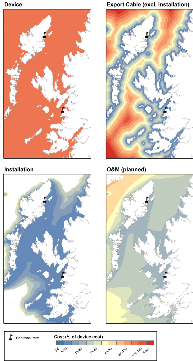
Figure 4: The four main project cost components which were considered for the case study. The export cable cost includes the capital cost only (the installation cost is included in the installation figure), the cable modelled as running to the nearest land point. The data are represented as factors of the device capital cost, to preserve confidentiality.
