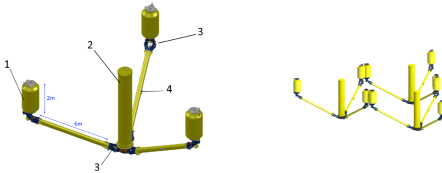
Figure 1: The Series-6 WaveNET wave energy device. Left: A single Squid unit, made up of buoyancy floats (1), a central riser (2), hydraulic pumping modules (3) and linking arms (4). Right: An array of three Squid units, arranged in a triangular formation.
