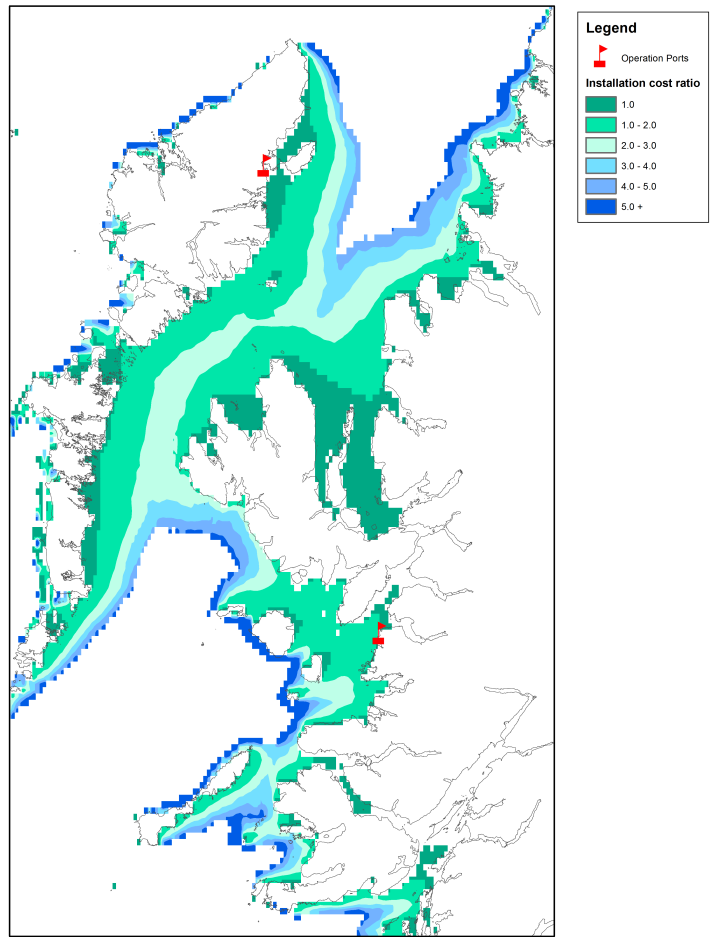
Figure 10: Ratio of project installation cost for a February installation divided by a July installation.
