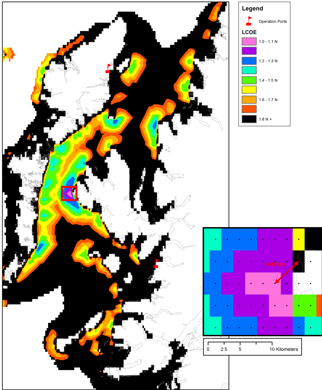
Figure 5: The LCOE over the domain for the baseline scenario. The lowest LCOE for the Series-6 device was found to be in the Little Minch, off the West Coast of Skye. The inset shows a close up of this area at the original data resolution (without interpolation) to illustrate the high spatial variability of the data. The data, represented as factors of an arbitrary constant N , have been non-dimensionalised to preserve commercial confidentiality.
