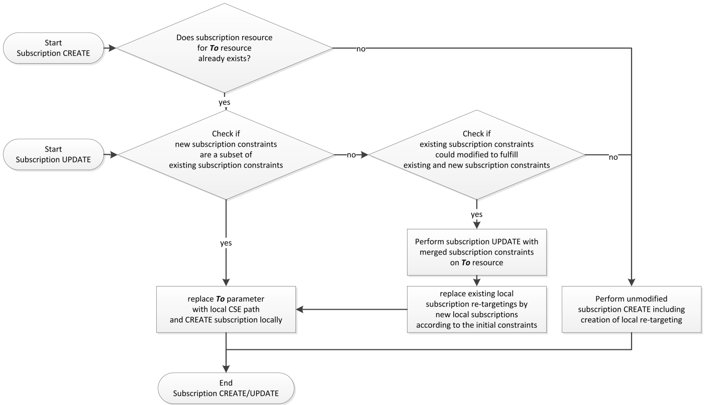
Fig. 4 Flowchart for aggregation of subscription constraints at local CSE.
