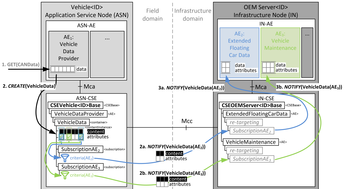
Fig. 2 An automotive scenario with current M2M data exchange capabilities
