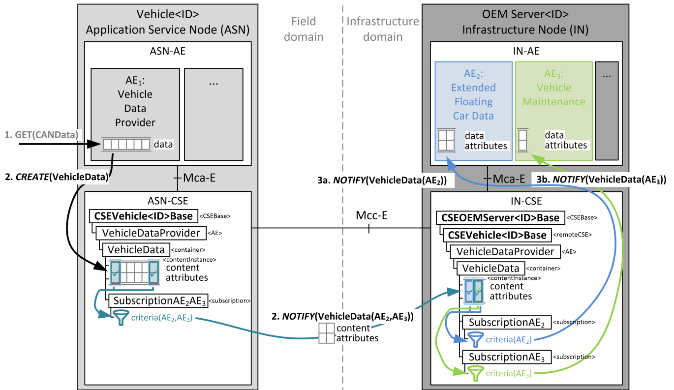
Fig. 5 An automotive scenario with enhanced M2M data exchange capabilities
