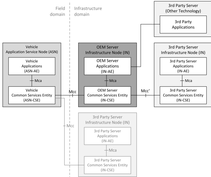
Fig. 1. Functional Architecture of an M2M-based Automotive Service Delivery Platform
