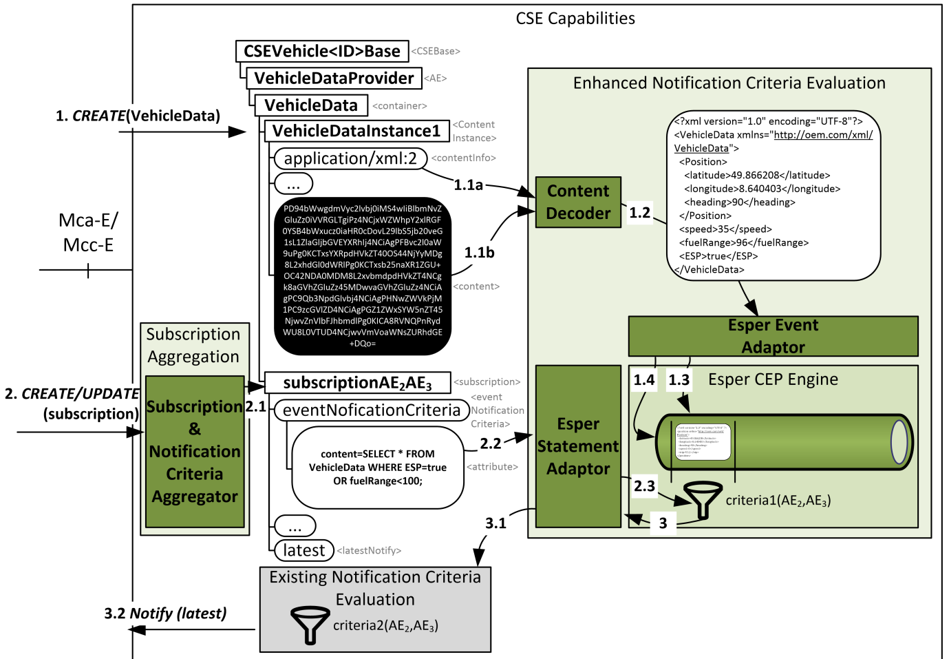
Fig. 3 Implementation of application-data-dependent notification criteria within the CSE
