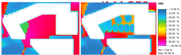
Figure 2: Microclimatic effect of different types of greenery on an average summer day (created with Envi-met)
