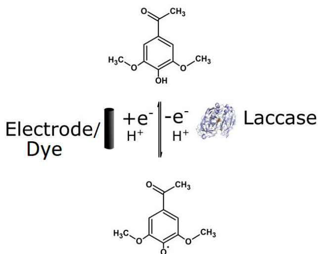
Figure 7. Electron transfer (ET) and Hydrogen atom transfer (HAT) oxidation mechanisms of acetosyringone mediated by laccase.
