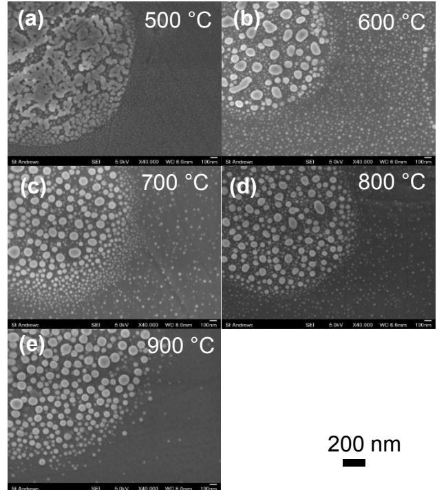
Figure 5. Morphology of Ni infiltrated LST44 when oxidized at 700 ^\circ\text{C} and then reduced in 5% \text{H}_2 at different temperature (From 500 ^\circ\text{C} to 900 ^\circ\text{C} ).
