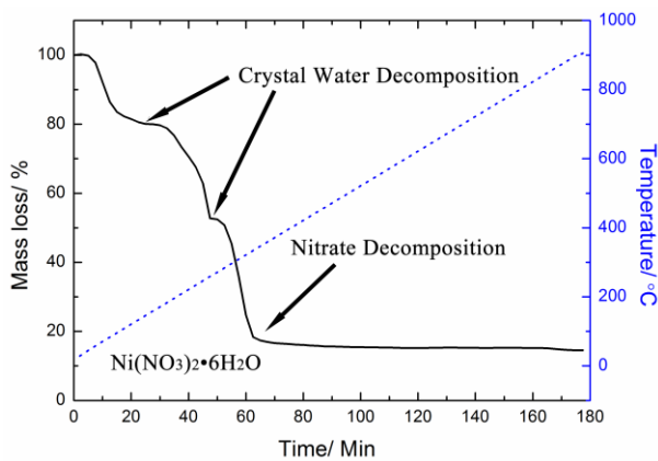
Figure 4. Mass change of \text{Ni}(\text{NO}_3)_2 \cdot 6\text{H}_2\text{O} heated from room temperature to 900 ^\circ\text{C} in air.
