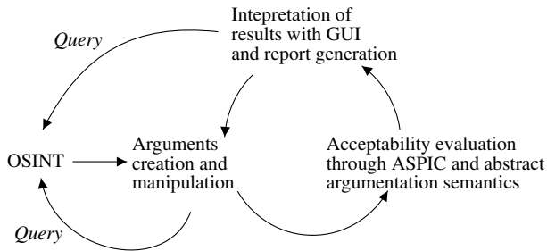
Figure 2. Overview of CISpaces.org functionalities.
