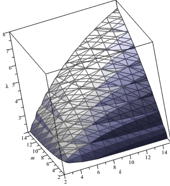
Figure 3: A plot depicting the surface consisting of values of m , k and \lambda for which \frac{\lambda(k-1)(m-2)}{(\lambda-1)k(m-1)} = 1 . By Theorem 4.1, if there exists an (n, m, k, \lambda) -SEDF then the point (k, m, \lambda) lies on or above the surface.
