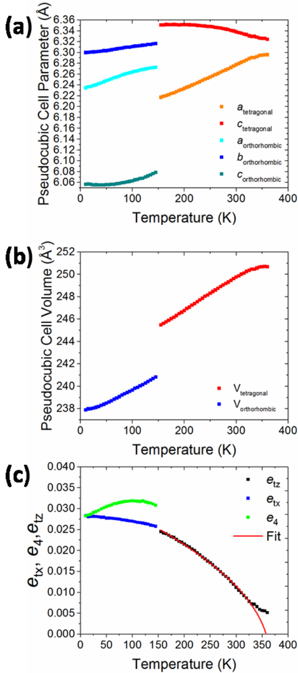
Figure 8: Variation of (a) cell parameters and (b) cell volume with temperature for \text{CD}_3\text{ND}_3\text{PbI}_3 in the orthorhombic, tetragonal and cubic regions. Due to the relatively fast ramp rate used and lack of equilibration time during the neutron diffraction experiment, the sample did not fully convert to cubic \text{CD}_3\text{ND}_3\text{PbI}_3 , hence only tetragonal cell parameters are shown in this temperature region. (c) Spontaneous strain obtained from lattice parameters over the full temperature range of the neutron diffraction experiments. The curve through data for e_{tz} represents a fit for e_{tz}^2 \propto (T_c - T) . The tetragonal-orthorhombic transition is strongly first order.
