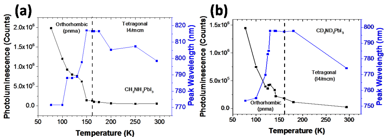
Figure 9: Photoluminescence wavelength (blue data points) and intensity (black data points) versus temperature for (a) CH 3 NH 3 PbI 3 and (b) CD 3 ND 3 PbI 3 . Dashed vertical lines represent the phase transition temperatures.
