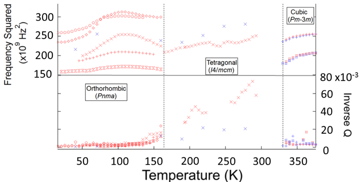
Figure 3: Variation of f^2 (representing elastic constants) and Q^{-1} (representing acoustic loss) as a function of temperature, for different resonance peaks in a single crystal of \text{CH}_3\text{NH}_3\text{PbI}_3 , scaled to be closer together for clarity. The phase transitions are shown by dotted lines. Blue and red points represent data collected on cooling and heating respectively.
