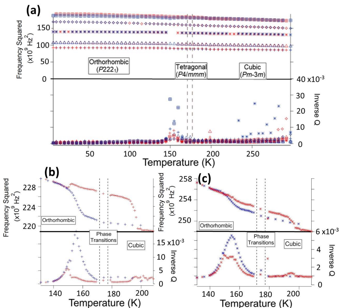
Figure 6: Variation of f^2 and Q^{-1} with temperature for the resonance peaks in RUS spectra from a single crystal of CH 3 NH 3 PbCl 3 . Dotted lines represent the expected phase transition temperatures. Blue points and red points represent values for the cooling sequence and the heating sequence respectively. (a) Variation of f^2 and Q^{-1} values over the full temperature range. (b,c) Variation of f^2 and Q^{-1} values for 480 and 510 kHz respectively over a narrower temperature range. f^2 values in (a) are scaled so that all data points fit on the same plot. The symbols representing the peaks in (b) and (c) represent the same peaks in part (a).
