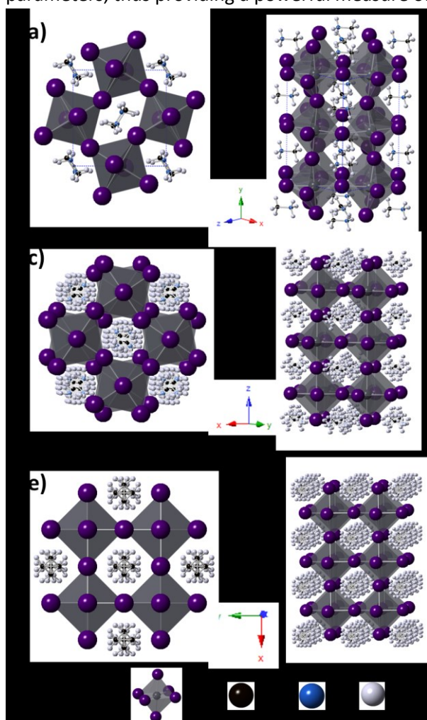
Figure 1: Structures adopted by \text{CH}_3\text{NH}_3\text{PbI}_3 as determined by Whitfield et al. [20] (a and b) Orthorhombic, Pnma , (c and d) tetragonal, I4/mcm and (e and f) cubic, Pm\bar{3}m . (a) ac plane, (c) ab plane.
