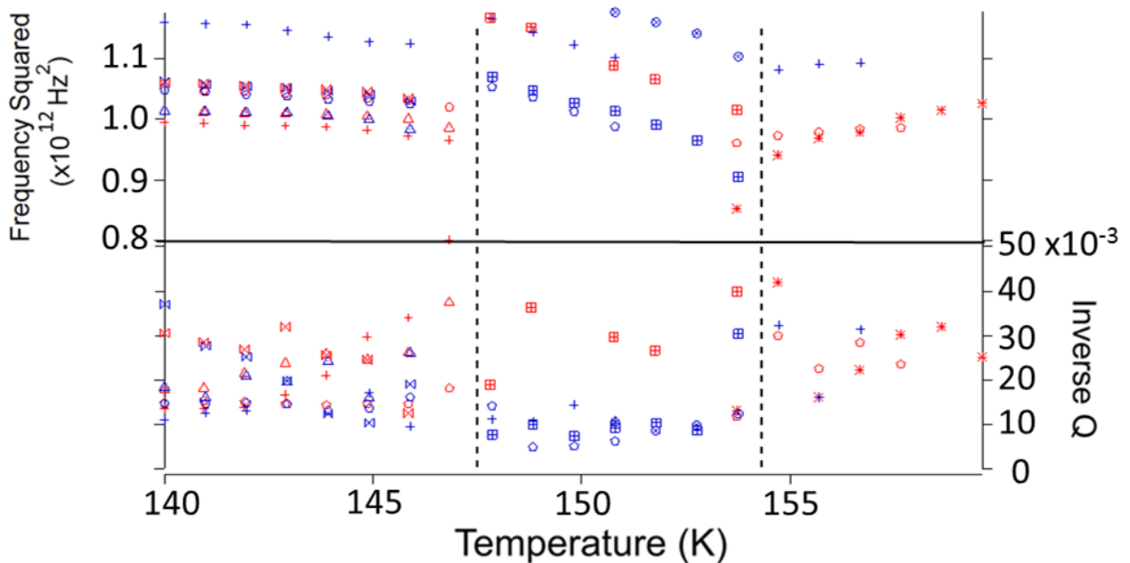
Figure 5: Variation of f^2 and Q^{-1} with temperature for \text{CH}_3\text{NH}_3\text{PbBr}_3 . Data were collected in a narrower temperature range using 1 K steps in the region around the expected orthorhombic-tetragonal phase transition. The dotted lines represent phase transitions. The peaks shown are in the 400-1200 KHz frequency range. Note that the Q^{-1} data display a relatively high degree of scatter because the resonance peaks become much more weakly defined at temperatures near to the phase transition.
