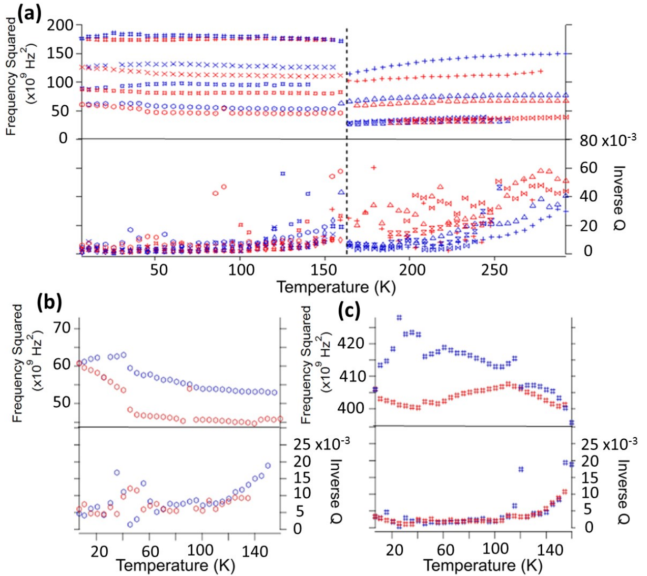
Figure 7: Variation of f^2 and Q^{-1} with temperature for over (a) the full temperature range (b) and (c) a narrower temperature range, for selected resonance peaks in RUS spectra collected from a single crystal of \text{CD}_3\text{ND}_3\text{PbI}_3 . (b) and (c) show the form of the anomalies in the evolution of f^2 for the selected resonance peaks and these may be indicative of an additional phase transition at \sim 40 K. The tetragonal – orthorhombic transition is marked with a vertical broken line. Data collected on cooling and heating are represented by blue and red points respectively.
