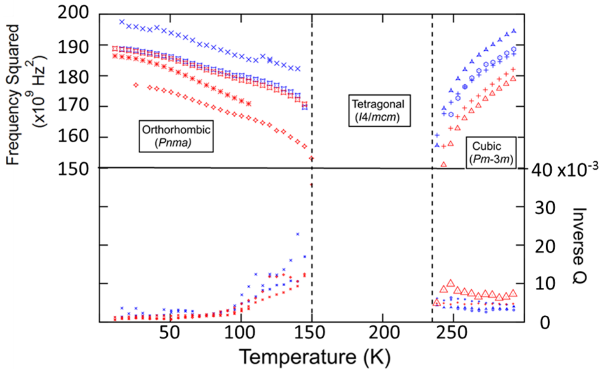
Figure 4: f^2 and Q^{-1} values for resonance peaks in spectra collected from a single crystal of \text{CH}_3\text{NH}_3\text{PbBr}_3 during cooling (blue) and heating (red). Vertical dashed lines represent phase transitions. Due to high attenuation, it was not possible to follow resonance peaks in spectra collected between \sim 150 and \sim 235 K, corresponding to the expected limits for the stability field of the tetragonal phase. All f^2 values have been scaled so that they fit on the same plot.
