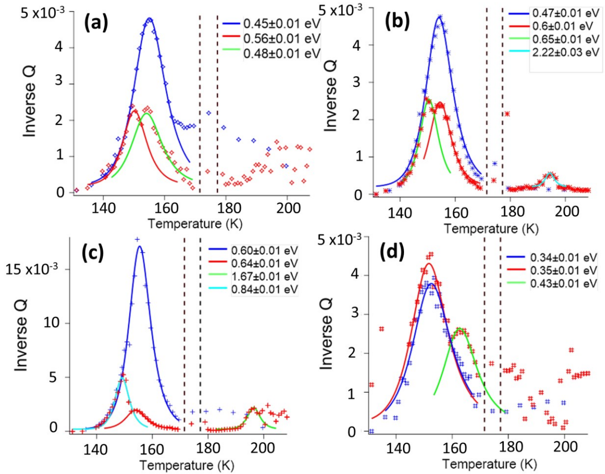
Figure 10: Fits of Equation 1 to selected loss peaks at (a) 1020 KHz, (b) 510 KHz, (c) 480 KHz and (d) 290 KHz, respectively, for resonances observed during cooling (blue) and heating (red). A constant baseline is removed from each data set prior to fitting. The values of E_a shown for each peak are under the assumption that r_2(\beta) = 1 . Activation energies for each fit are shown in the legend.
