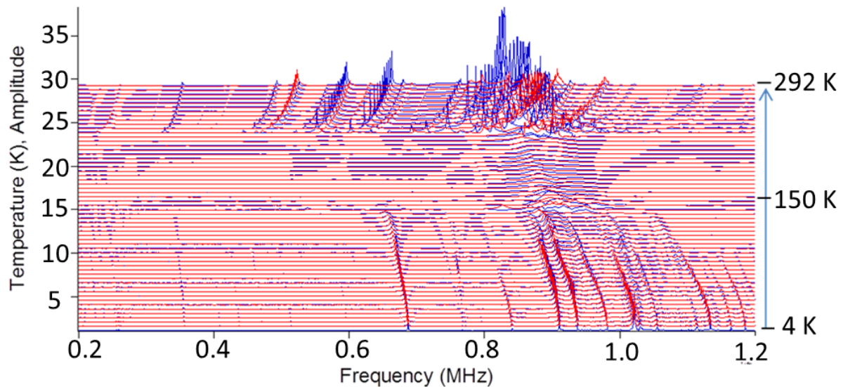
Figure 2: Primary RUS spectra from a single crystal of \text{CH}_3\text{NH}_3\text{PbI}_3 . The spectra have been offset up the y-axis in proportion to the temperature at which they were collected, such that the uppermost spectrum was collected at \sim 300 K, and the lowermost one at \sim 5 K. Individual spectra were collected in 5 K intervals during cooling (blue lines) and heating (red lines).
