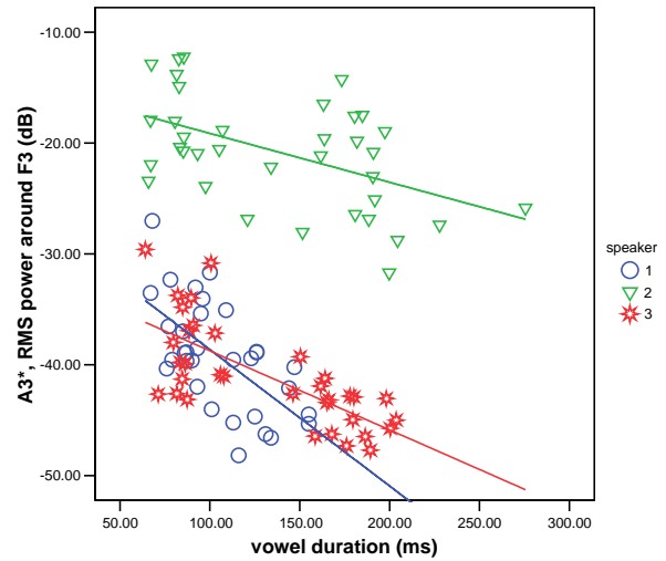
Figure 3 Correlation between the measure A3* (dB) and the duration of /ʉ/ (ms) for the three SSE speakers.
