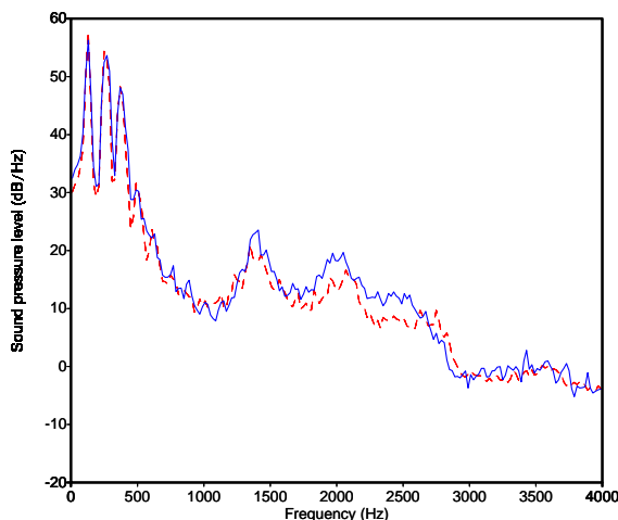
Figure 2 Long-term average spectrum of all short (blue plain line) and all long (red dashed line) tokens of [ʉ] produced by Speaker 3 (male).
