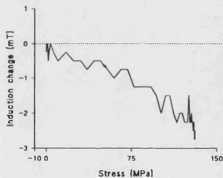
Figure 5.17: Induction deflection observed from HY80(2) after a demagnetization process.
