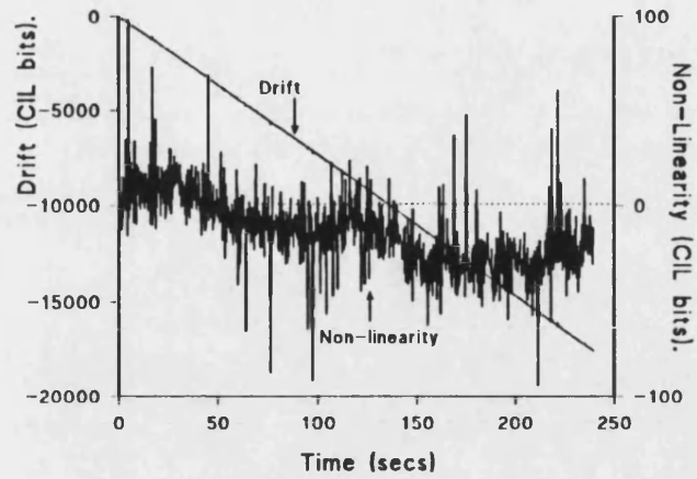
Figure 5.8: Integrator drift against time. The departure from linearity is indicated on the right-hand scale. Specimen (Fe(2)) in situ., field held constant.
