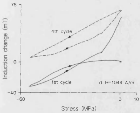
Figures 6.7 (Top left): Vacuum annealed HY80(2): main magnetic hysteresis loop. Induction changes with compressive cycles at indicated points on the initial induction curve are as indicated. For clarity, only the first and fourth induction changes are shown.
