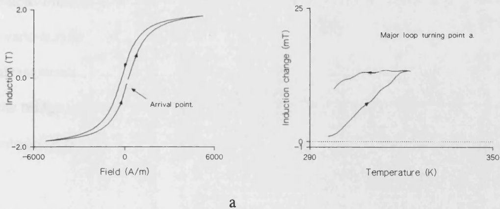
Figure 5.15 a & b: Induction change induced by increasing the temperature from a major loop point for Fe(2). a. Arrival at major loop point. b. Induced change.
