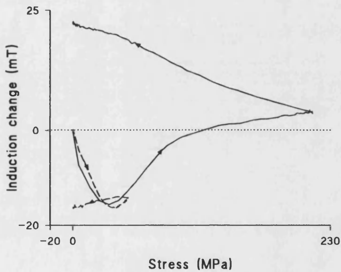
Figure 6.45. a. (Top) Stress-induced induction changes with increasing magnitude of compression from a minor loop point. b. Stress-induced induction changes for low and high tensile loads from a minor loop point. These results prove conclusively that the sense of irreversible induction changes on minor loops is stress-magnitude dependent.
