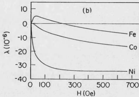
Figures 3.1 (a). (Left). The longitudinal magnetostrictions of iron along the principal crystal directions. (b). The net strain of ferromagnetic isotropic polycrystalline specimens. The inversion of specimen strain (contraction at higher fields) commonly demonstrated by iron-based polycrystalline materials should be noted. (Bozorth, 1951).
