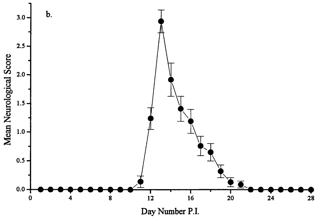
Figure 3.1 Characterisation of actively induced EAE.
