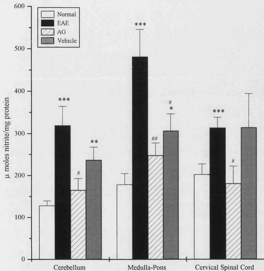
Figure 6.4 Effect of AG administration on nitrite levels in CNS cytosol
