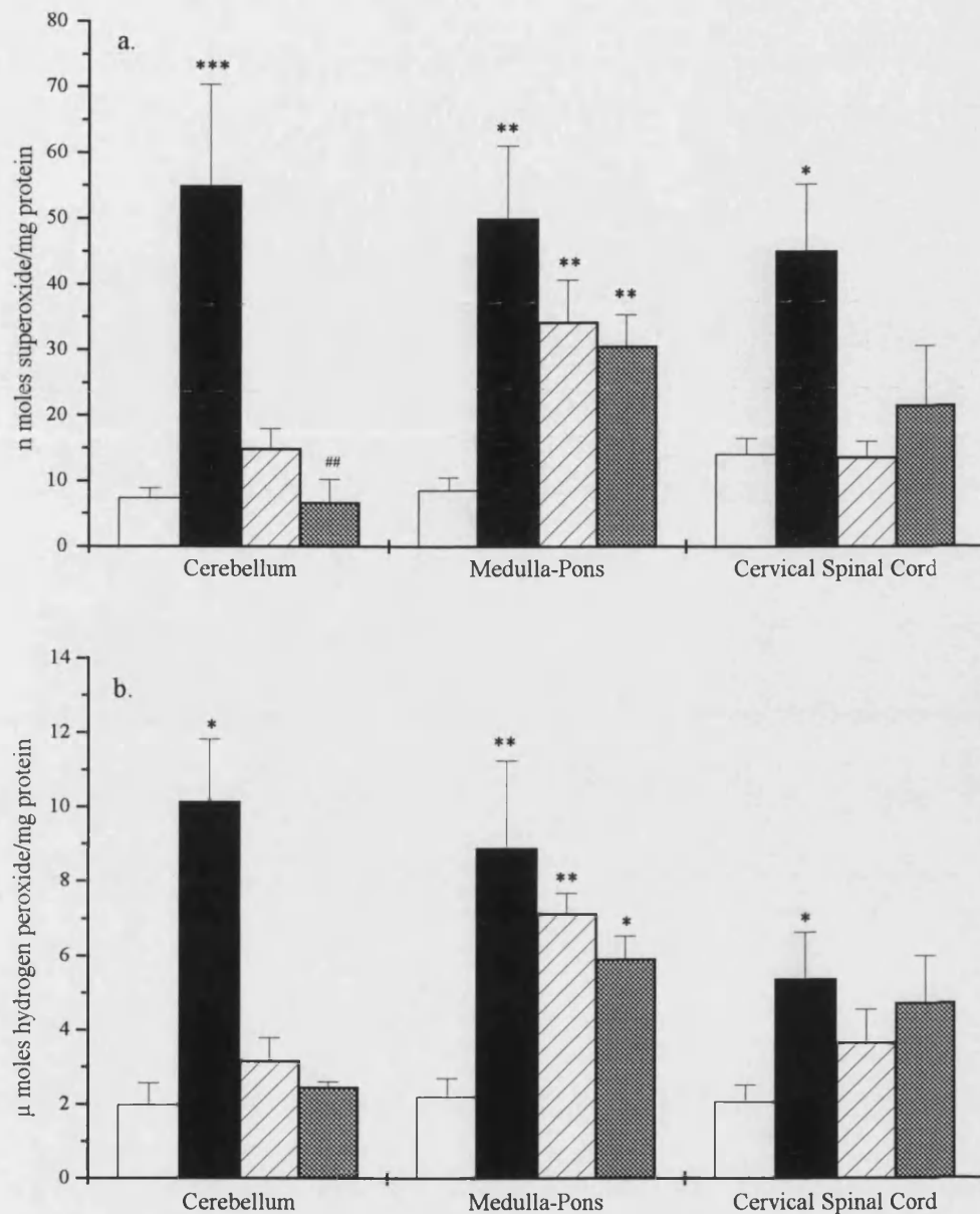
Figure 5.9 Effect of CsA administration on ROS levels in CNS cytosol CNS cytosol was prepared from the cerebellum, medulla-pons and cervical spinal cord tissues.
