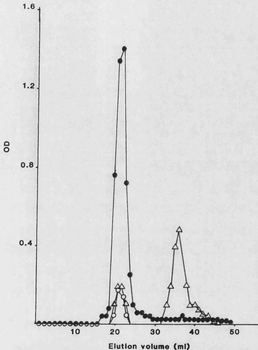
Figure 4.4.1 Elution profile of neuraminidase treated AChR on Sephadex G25 column (1.8cm x 82cm). The column was eluted with 10mM ammonium acetate, pH 7.4, and fractions of 3ml were collected with a flow-rate of 30ml/h. (●) Protein (Lowry et al., 1951), (○) hexose sugars (cysteine/sulphuric acid assay), (Δ) sialic acid (thiobarbituric acid assay).
