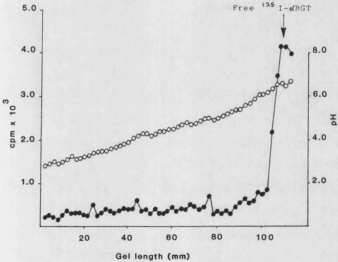
Figure 4.5.2 Isoelectric focusing gel of AChR following incubation with 125 I-αBGT in the presence of 25mM benzoquinonium chloride.
