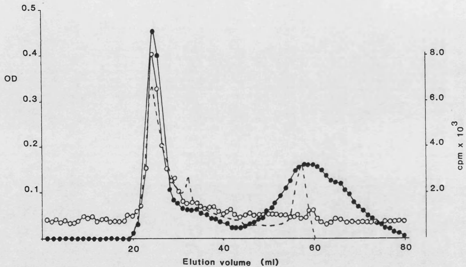
Figure 4.3.1 Chromatography of AChR (1.5 - 2.5 mg) on Sephacryl S200 (superfine) column (1.5cm x 30cm). The column was eluted with potassium phosphate buffer, 10mM, pH 7.4 containing 0.3M NaCl. Fractions of 1ml were collected with a flow-rate of 60ml/h. (●) Protein (280nm), (- - -) protein (Lowry et al, 1951), (o) toxin binding activity.
