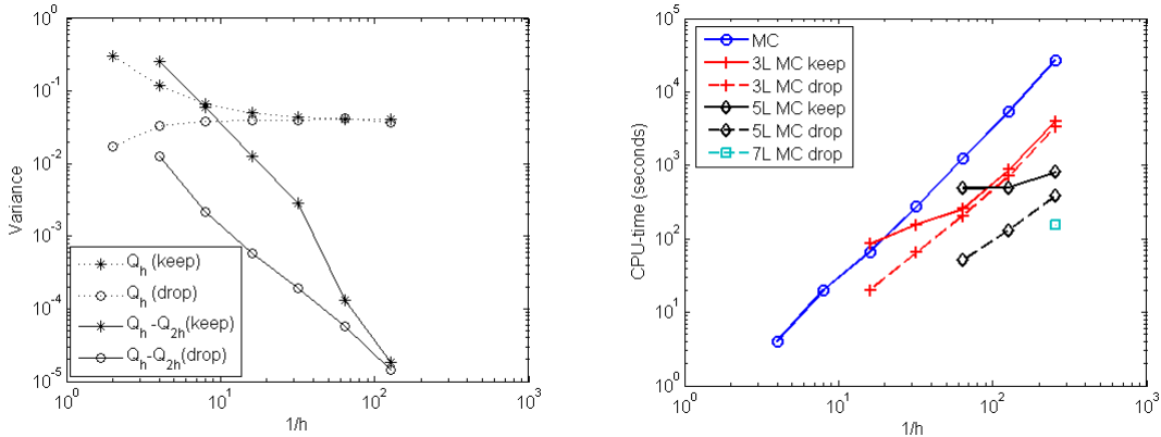
Figure 4-8: Left: Plot of \mathbb{V}[M_\omega^{(4)}(u_h)] and \mathbb{V}[M_\omega^{(4)}(u_h) - M_\omega^{(4)}(u_{2h})] , for (3.19) with d = 2 , \lambda = 0.1 , \sigma^2 = 1 , \psi = x_1 , R_\ell = 4h_\ell^{-1} , h^* = 1/256 and R^* = 1024 . Right: Plot of cost CPU-time versus 1/h for a fixed tolerance of the sampling error of \delta = 10^{-3} , for the same model problem.
