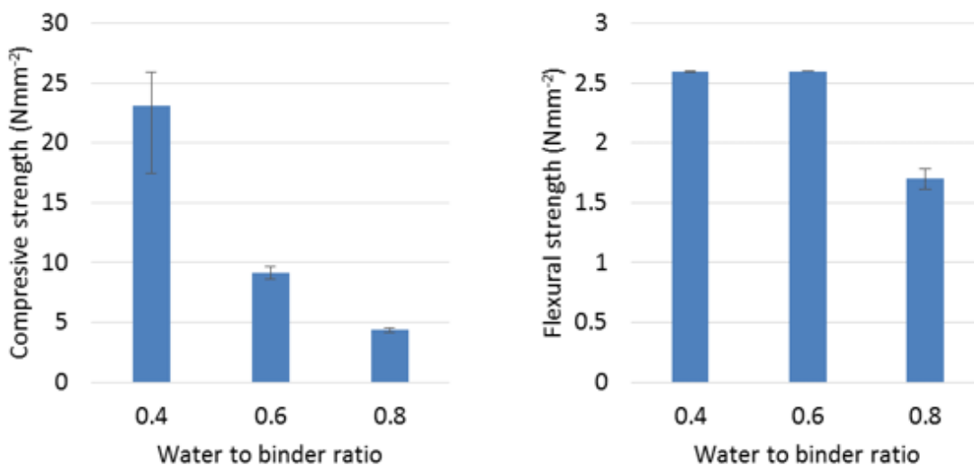
Figure 4.13: The compressive and flexural strength of Tradical Thermo binder at three water to binder ratios at 28 days.
