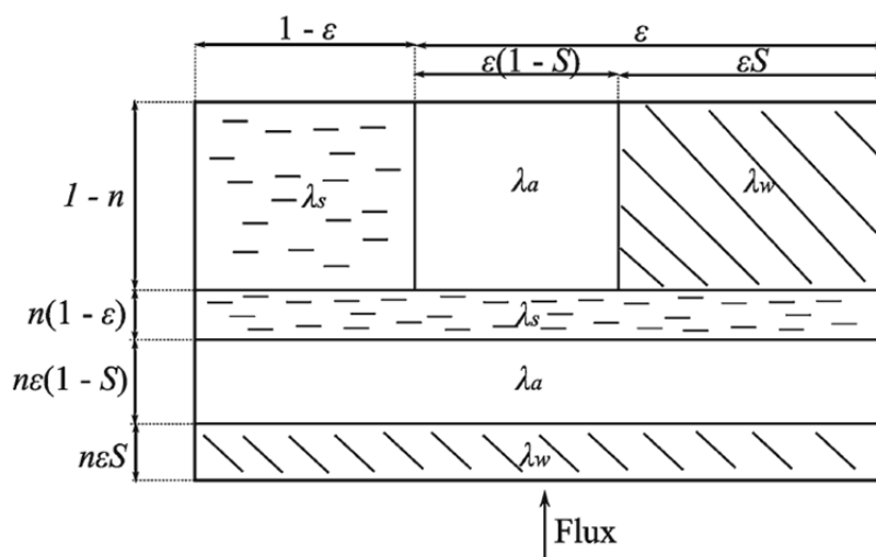
Figure 2.14: Diagrammatic representation of a three phase Krischer thermal conductivity model as presented by (Pierre et al., 2014).
