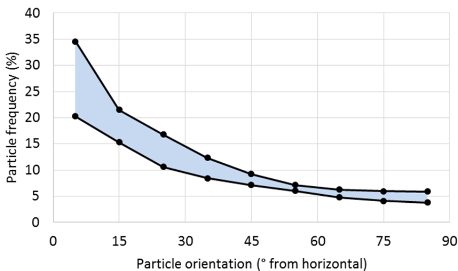
Figure 3.10: The window of frequency orientation plots obtained using the range of image processing on perpendicular, two dimensional digital images of pre-treated standard mix hemp-lime.
