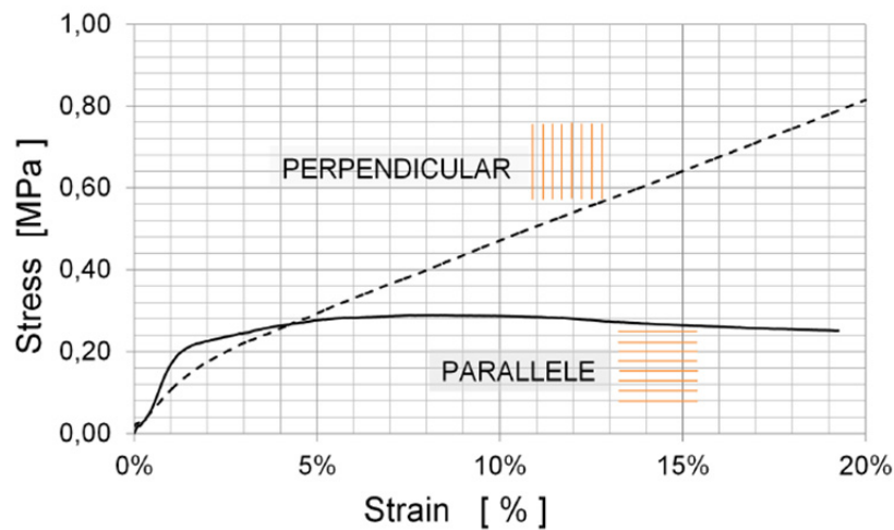
Figure 2.3: Parallel and perpendicular to compaction loading of hemp-lime as presented by (Kashtanjeva et al., 2015).
