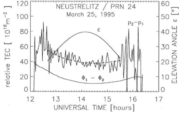
Figure 3. Differential pseudo-ranges and carrier phases relative to satellite PRN24 reproduced over Neusterlitz (Germany) on the 25th of March 1995. The dashed line shows how the least square method over imposed the two differentials in order to have a calibrated measurement [Jakowski, 1996].
