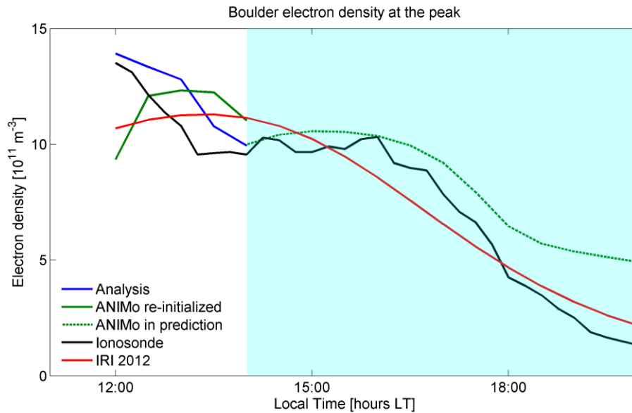
Figure 39. Comparisons of electron densities at the peak by ANIDAS method A (blue), by re-initialized ANIMo (green), by IRI-2012 (red) and measured by ionosonde (black) for the now-casting case study (29 th of December 2011 from 1200 to 1400 LT (1900 to 2100 UT)) and by ANIMo (dashed green) in forecasting (29 th of December 2011 from 1400 to 2000 LT (2100 to 0300 UT)), highlighted in light blue over Boulder.
