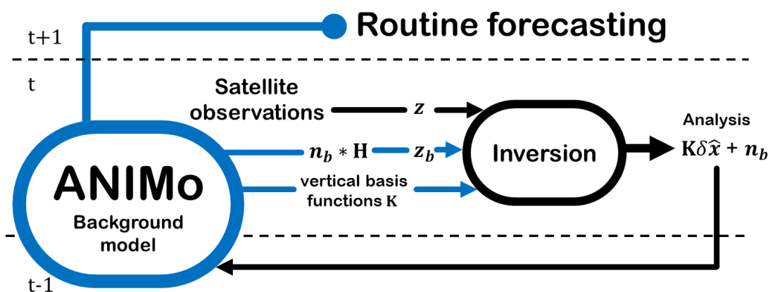
Figure 23. Simplified diagram of the principal components of ANIDAS scheme used in an iterative manner. The letter t indicates time step.
