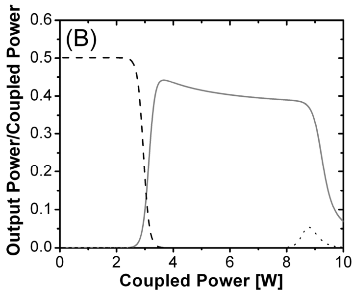
Fig. 6.1 (A) Theoretical conversion efficiency from the input pump power to the output power at the first rotational Stokes wavelength as a function of the propagation length and the input power. (B) Calculated output power ratio to the total input power at the pump (dashed line), first Stokes (solid grey line), second Stokes (dotted line) as a function of the coupled power for 30m of HC-PCF. The anti-Stokes output power is 10^{-6} weaker than the pump and Stokes lines and is not represented.
