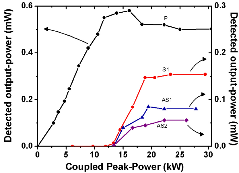
Fig. 8.5 Detected output power from the pump (black circles and line), first Stokes (red circles and line), first anti-Stokes (blue triangles and line) and second anti-Stokes components (purple diamonds and line), as a function of the coupled peak power. Each component is taken from a fraction of the output beam diffracted on a grating.
