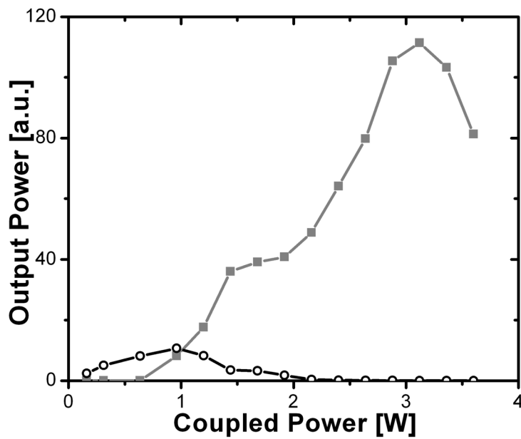
Fig. 6.8 Output power vs coupled input power for the pump (circles and black line) and S_{00}(1) (grey squares and line) when using FBGs to form a cavity. The drop in Stokes intensity above 3W is due to conversion to second Stokes.
