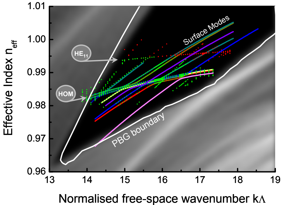
Fig. 1.4 DOPS diagram of the region of the PBG falling below the vacuum line ( n_{eff}=1 ). Inside the PBG, defect-guided modes can be calculated and their trajectories identified using the plane wave method [10]. The trajectory of the core-guided fundamental ( HE_{11} ) mode and other high order modes (HOM) are identified, as well as surface modes (solid lines). Anti-crossing events between core-guided and surface modes are also observed.
