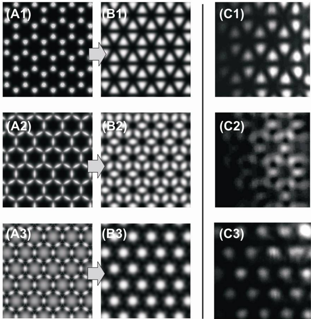
Fig. 2.8 (A) Calculated near-field profile for (A1) the apex mode, (A2) strut mode and (A3) airy mode. (B) Corresponding Fresnel zone mode patterns. The position of the diffraction pattern is 1.8\lambda , 1.5\lambda and 2.0\lambda away from the fibre for the three modes, respectively. (C) Observed Fresnel zone mode patterns for a wavelength of 950nm, 750nm and 700nm in a HC-PCF guiding around 800nm. The pattern positions, relative to the end of the fibre, are in the range of 4-5 \mu m.
