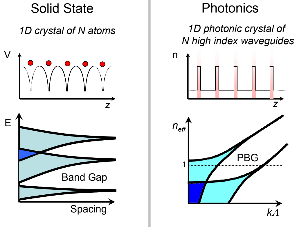
Fig. 2.4 Similarities between the tight binding model describing the formation of electronic band gap in solid state physics (left) and the coupled resonator picture describing the formation of photonic band gap in photonic crystals (right).
