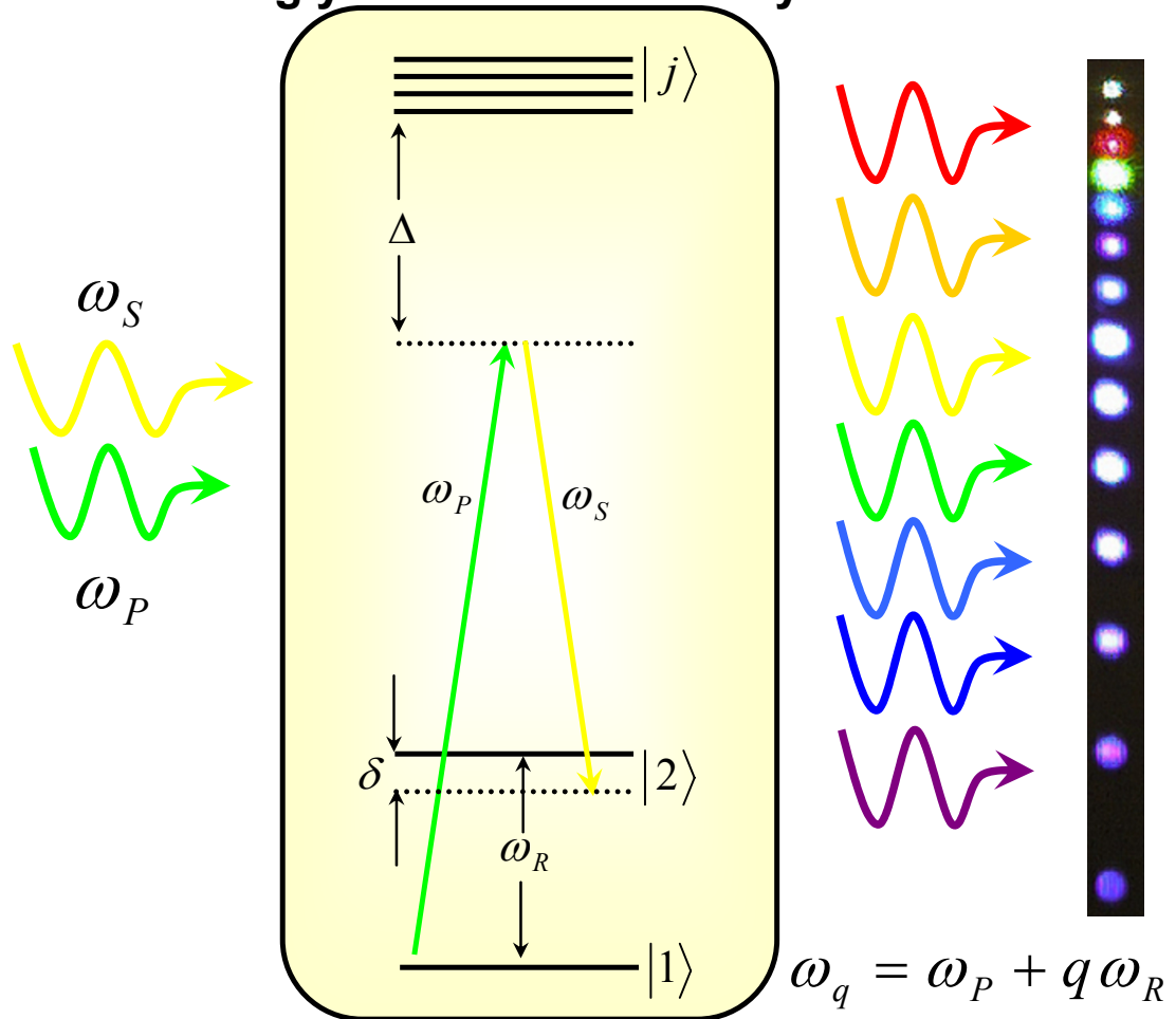
Fig. 1.12 Raman sidebands generation when conditions on coherence and adiabaticity are met. (Right) Typical resulting Raman sidebands in D_2 (from [53])
