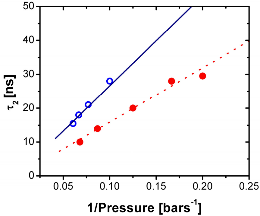
Fig. 5.7 Experimental \tau_2 as a function of the inverse of the \text{H}_2 pressure for 15m (red dots) and 25m (blue circles). The theoretical evolution is represented in dotted red and solid blue lines, respectively.
