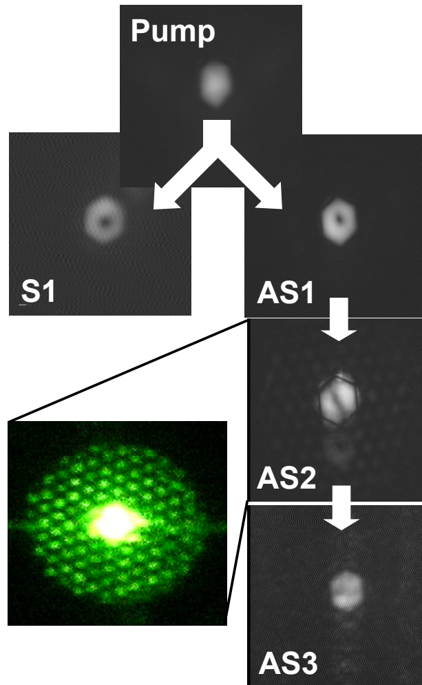
Fig. 8.4 Near field profile of the output from the H_2 -filled Kagomé fibre. The Stokes (S) and anti-Stokes (AS) frequencies are separated from the pump by means of a diffraction grating. The transverse profile of AS2 is also shown in colour (left hand-side picture). This anti-Stokes line lies in the low transmission band of the Kagomé fibre. One could see that the AS2 light also couples to cladding holes via linear phase-matching between the core-mode and the cladding hole-modes.
