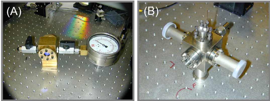
Fig. 3.2 (A) Brass gas control chamber for loading of high pressure gas and (B) stainless steel gas control chambers specially designed for vacuum applications
