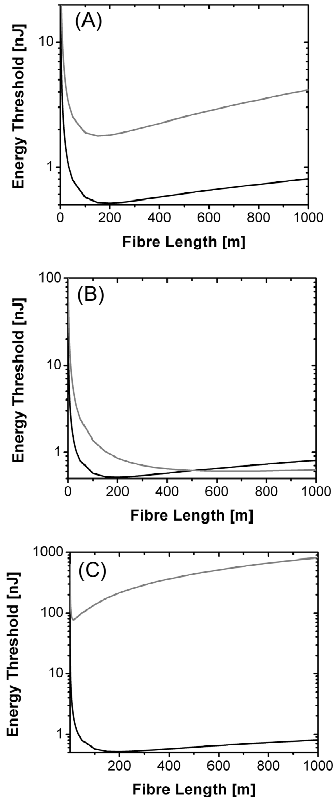
Fig. 4.10 (A) Energy threshold as a function of fibre length for the steady state (black line) and transient regime (grey line). (B) Steady state energy threshold as a function of fibre length for a HC-PCF guiding at 1064nm (black line) and one guiding at 1550nm (grey line). (C) Steady state energy threshold as a function of fibre length for the HC-PCF guiding at 1064nm (black line) and a Kagomé fibre (grey line). Details of the parameters used for the calculations are given in the text.
