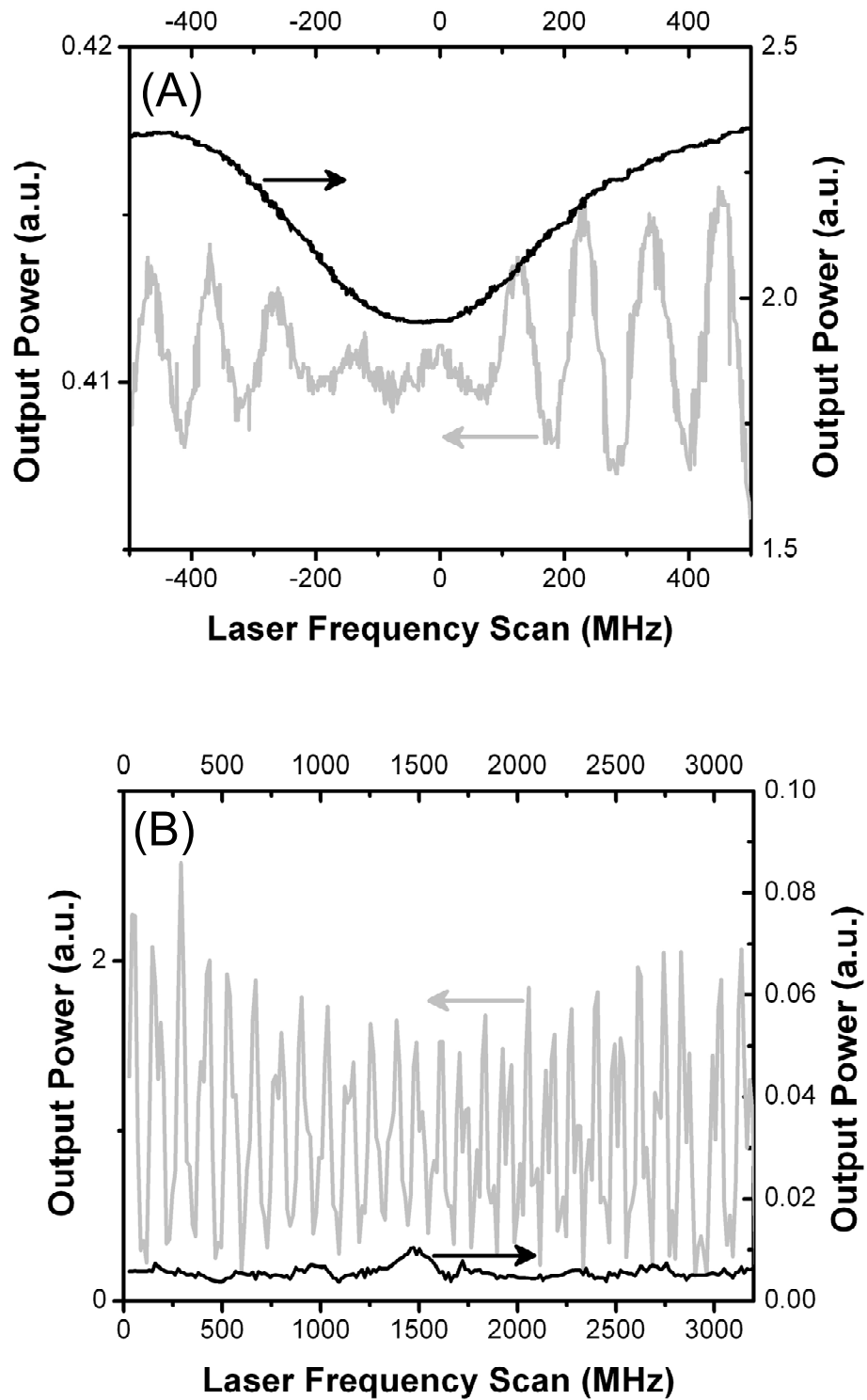
Fig. 3.19 (A) Reflected output power of a C_2H_2 gas-cell with perpendicular cleave versus laser detuning around the absorption line P13 of C_2H_2 (grey line). The interference pattern makes the detection of the line (black line) very difficult. (B) Output reflected power for the perpendicular (grey line) and the angle (black line) spliced HC-PCF gas cell. The fringes amplitude reduction is accompanied by a power reduction also due to the angle cleave.
