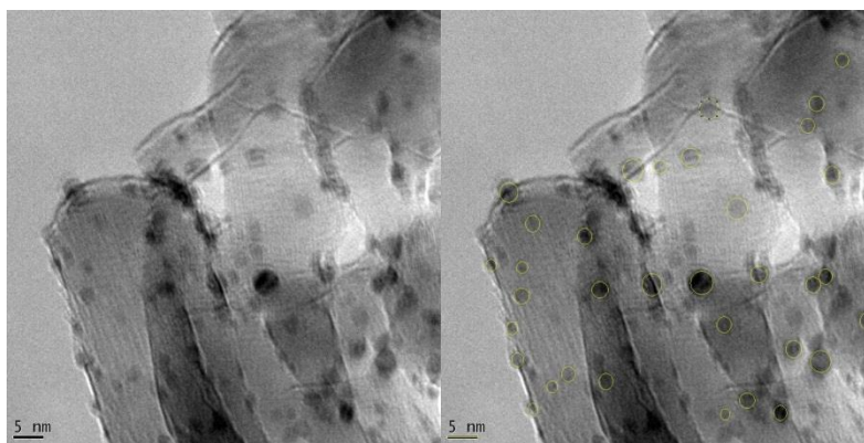
Figure 7.5 - TEM image of TiPt7.1%IE showing a representation of particles that are selected for sizing. The diameter of the yellow circle is used as the value for the particle size.
