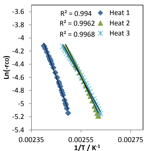
TiPt5.0%IE
