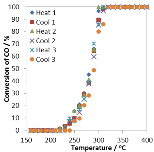
TiPt0.6%Pre-NP
