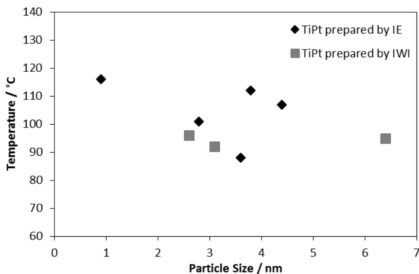
Figure 7.8 – Average particle size measured by CO chemisorption as a function of the temperature of the maximum peak in TPR experiments.
