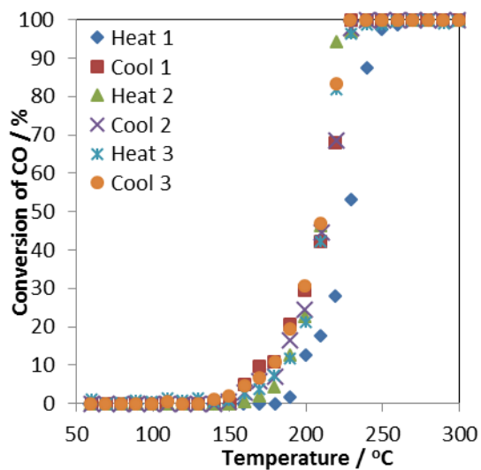
TiPt4.8%IWI
