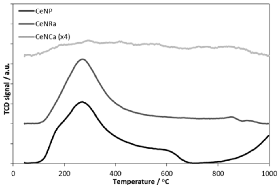
Figure 5.4 - Temperature programmed treatment under inert atmosphere of CeNP, CeNR A and CeNC A . Run between ambient and 1000 °C under helium at 30 mL min -1 , signal adjusted for weight. TCD signal is inverted.
