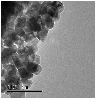
Figure 4.2 - TEM image and histogram of particle diameters of ceria nanoparticles, CeNP. Synthesised at 5 M NaOH and 70 °C with particle diameters measured from several images at different locations.
