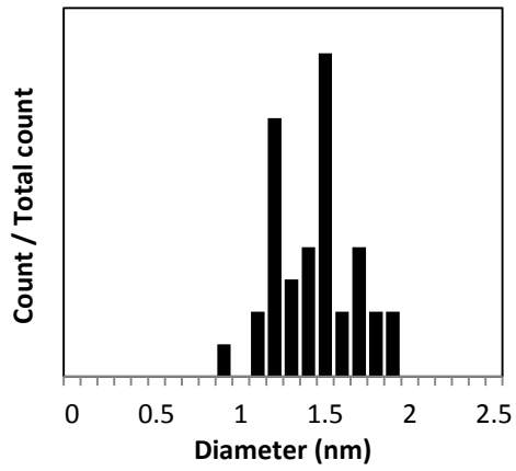
TiPt4.8%IWI
