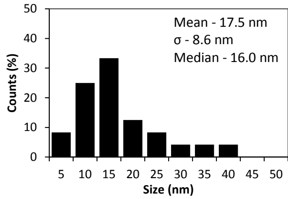
Figure 4.2 - TEM image and histogram of particle diameters of ceria nanoparticles, CeNP. Synthesised at 5 M NaOH and 70 °C with particle diameters measured from several images at different locations.
