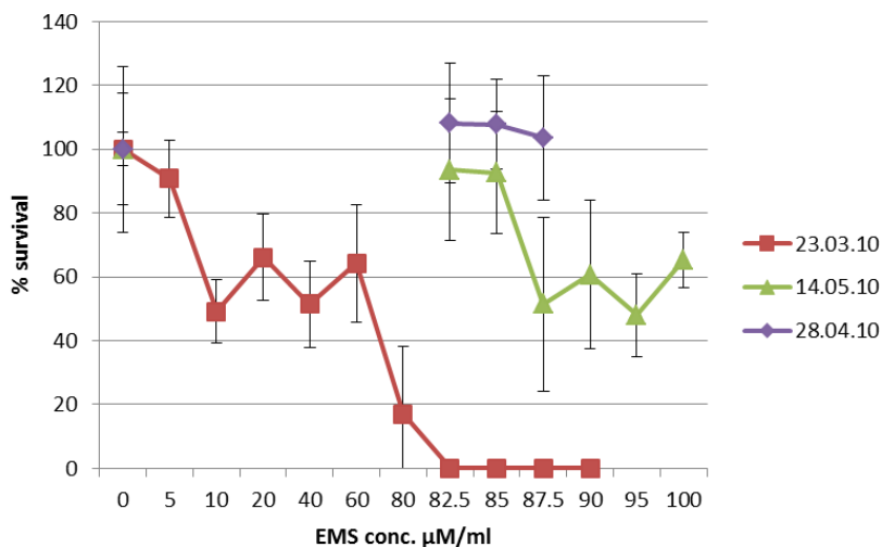
Figure 4.2: Replicates of EMS mutagenesis calibration curves for C. vulgaris , using various concentrations of EMS over a 10min exposure.
