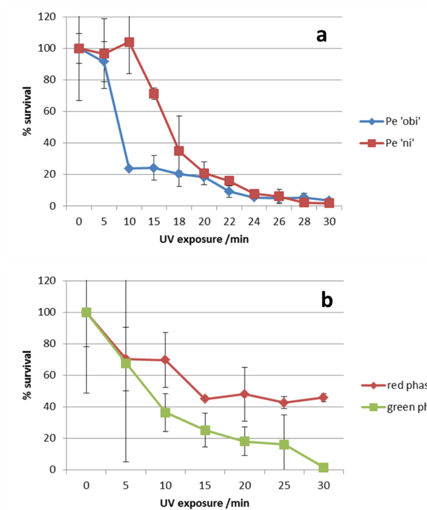
Figure 4.5: UV mutagenesis calibration curves for (a) P. ellipsoidea 'obi' and 'ni' and (b) H. pluvialis over different exposure periods. Survival values (colony counts) are given as a percentage compared to the control from plated aliquots of mutagenized culture. Three replicates of each were performed, error bars = S.D.
