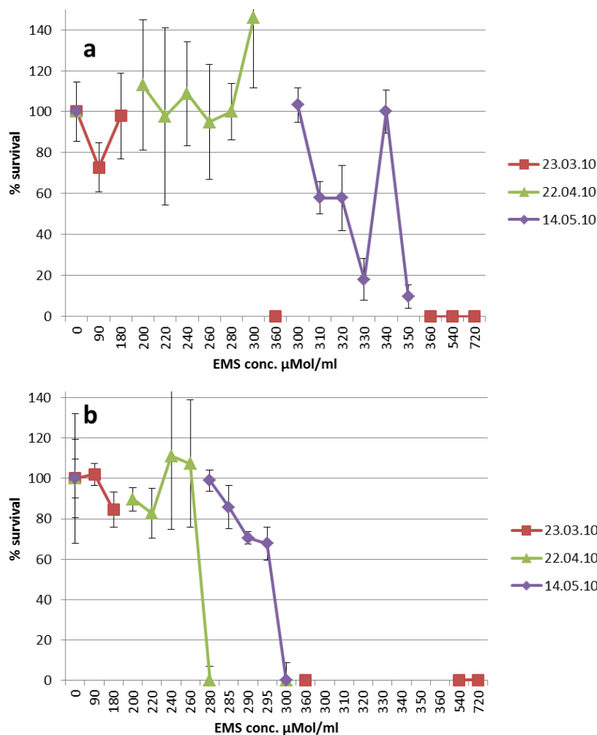
Figure 4.3: EMS mutagenesis calibration curves for P. ellipsoidea (a) ‘obi’ and (b) ‘ni’, using various concentrations of EMS over a 10min exposure. Survival values (colony counts) are given as a percentage compared to the control from plated aliquots of mutagenized culture. For each concentration five replicate agar plates were prepared, error bars = S.D. Each series was intended as a repeat experiment.
