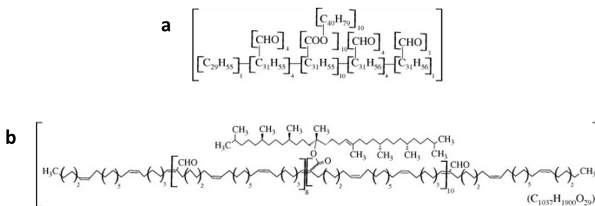
Figure 3.1: (a) Simplified representation of the macro-structure of algaenan and (b) expanded atomistic model of algaenan of Botryococcus braunii race L.
