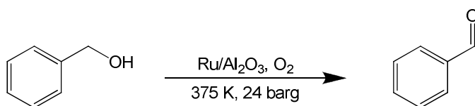
Scheme 2.3 Oxidation of benzyl alcohol with molecular oxygen.
