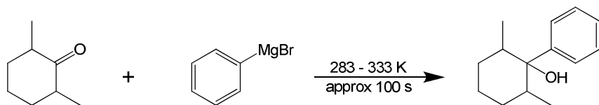
2,6-dimethylcyclohexanone
