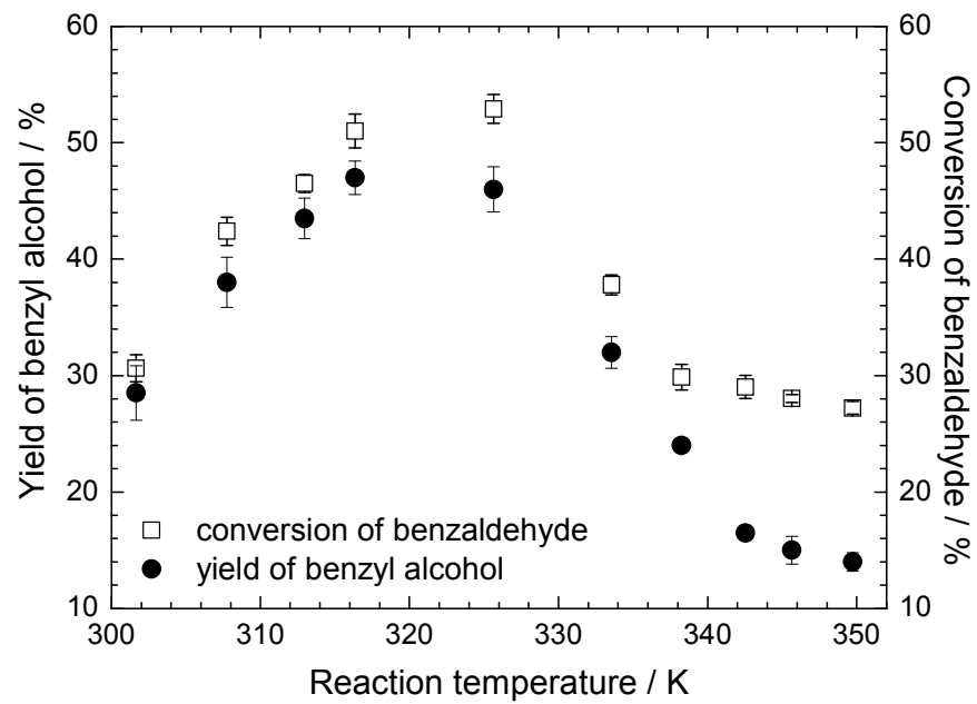
Fig. 3.8 Yield of benzyl alcohol and benzaldehyde conversion in the compact reactor as a function of reaction temperature. P = 8 barg, F_{\text{Liquid}} = 1.46 \text{ kg m}^{-2} \text{ s}^{-1} , F_{\text{Gas}} = 2.66 \times 10^{-3} \text{ kg m}^{-2} \text{ s}^{-1} , C_{\text{Substrate}, 0} = 0.2 \text{ mol L}^{-1} .
