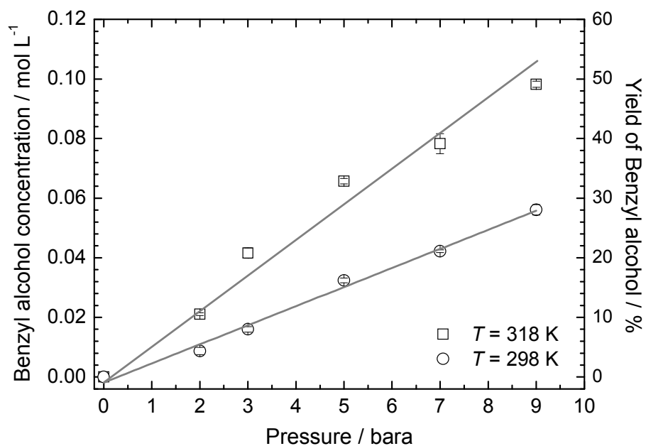
Fig. 3.5 Effect of the absolute pressure on the production of benzyl alcohol. F_{\text{Liquid}} = 1.46 \text{ kg m}^{-2} \text{ s}^{-1} , F_{\text{Gas}} = 2.66 \times 10^{-3} \text{ kg m}^{-2} \text{ s}^{-1} , C_{\text{Substrate}, 0} = 0.2 \text{ mol L}^{-1} .
