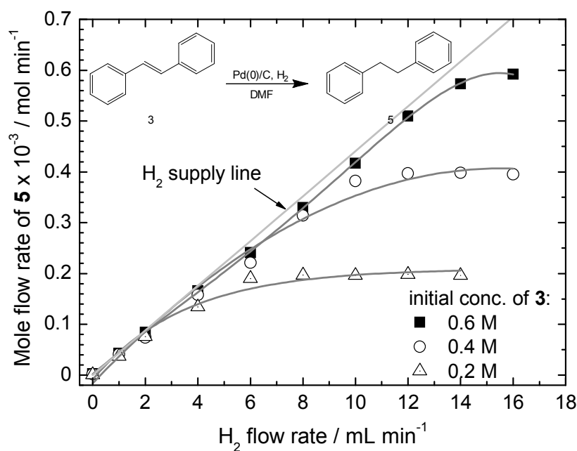
Fig. 5.6 Continuous alkene hydrogenation in the compact reactor. Reaction conditions: T = 397 K; P = 8 barg; F_{\text{Liquid}} = 1 mL min -1 ; two channels in series; approx. 0.9 g catalyst in the two channels.
