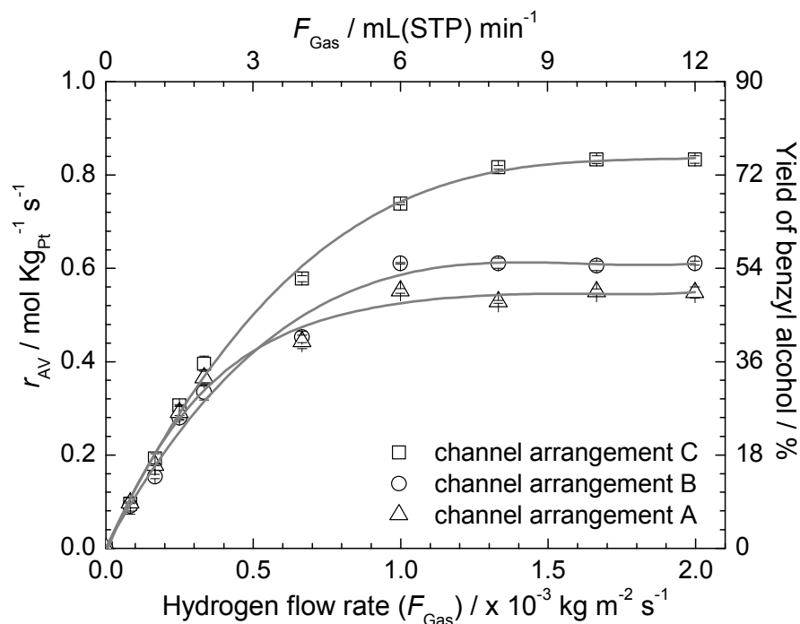
Fig. 3.13 Benzyl alcohol yield against gas flow-rate for different hydrogen injection strategies. P = 8 barg, T = 318 K, F_{Liquid} = 1.46 kg m^{-2} s^{-1} , C_{Substrate, 0} = 0.2 mol L^{-1} .
