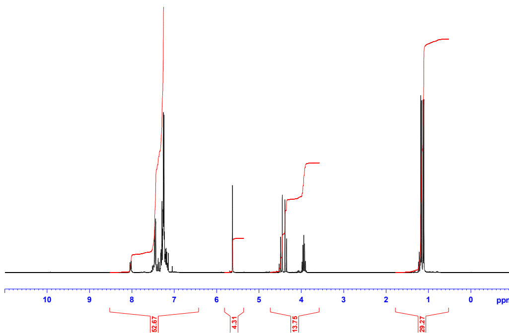
Fig. a.4 1 H NMR spectra of the byproduct in benzaldehyde hydrogenation.
