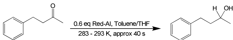
benzyl acetone
