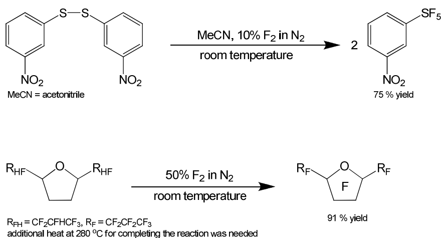
Scheme 2.2 Fluorination and perfluorination reactions requiring F_2 addition.
