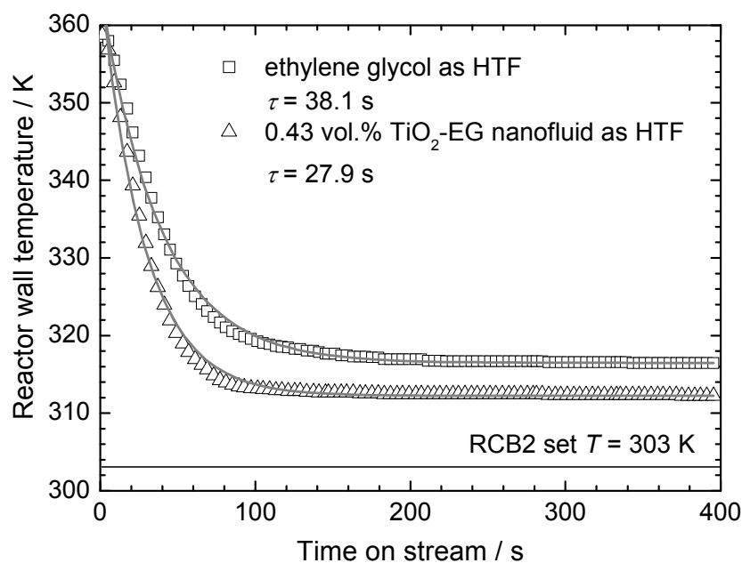
Fig. 4.11 Comparison of the temperature profiles of the quenching experiment based on EG and 0.43 vol.% TiO 2 -EG nanofluid. Symbols – experimental data points, solid lines – model fit curves.
