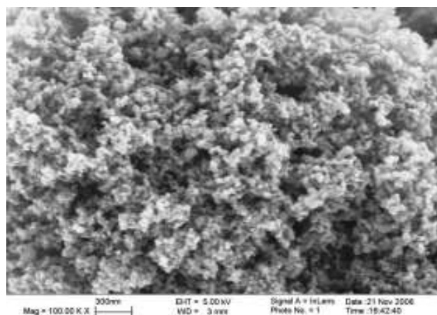
Fig. 4.2 SEM image of TiO 2 nanoparticles as received. Adopted from ref. 36.
