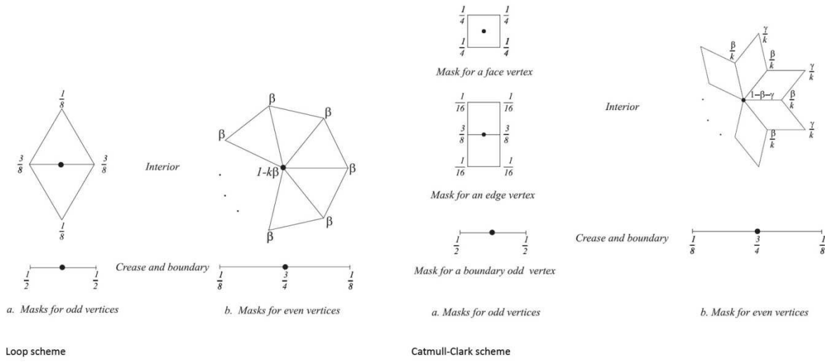
Figure 15 Subdivision rules for Loop(left) and Catmull-Clark (right) and schemes. Graphics courtesy of Schröder et al. (2009) For the Loop scheme, \beta = \frac{3}{16} if the vertex valence val is 3, and \beta = \frac{3}{8} val otherwise are used. For Catmull-Clark, \beta = \frac{3}{2} val and \gamma = \frac{1}{4} val .
