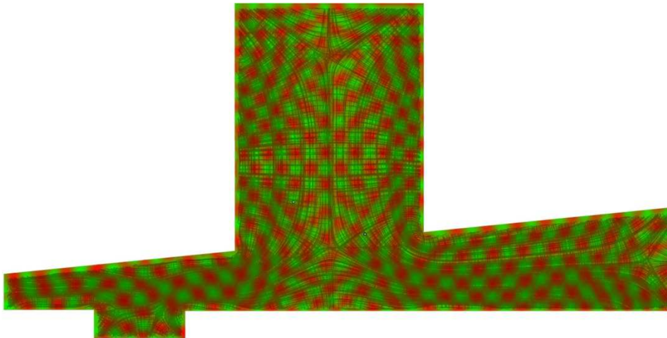
Figure 13 Wave function on glass goaf model, with curvature field streamlines overlaid. The function converged nicely over the central section but the wavelength is too long to capture the additional detail in the bottom left corner.
