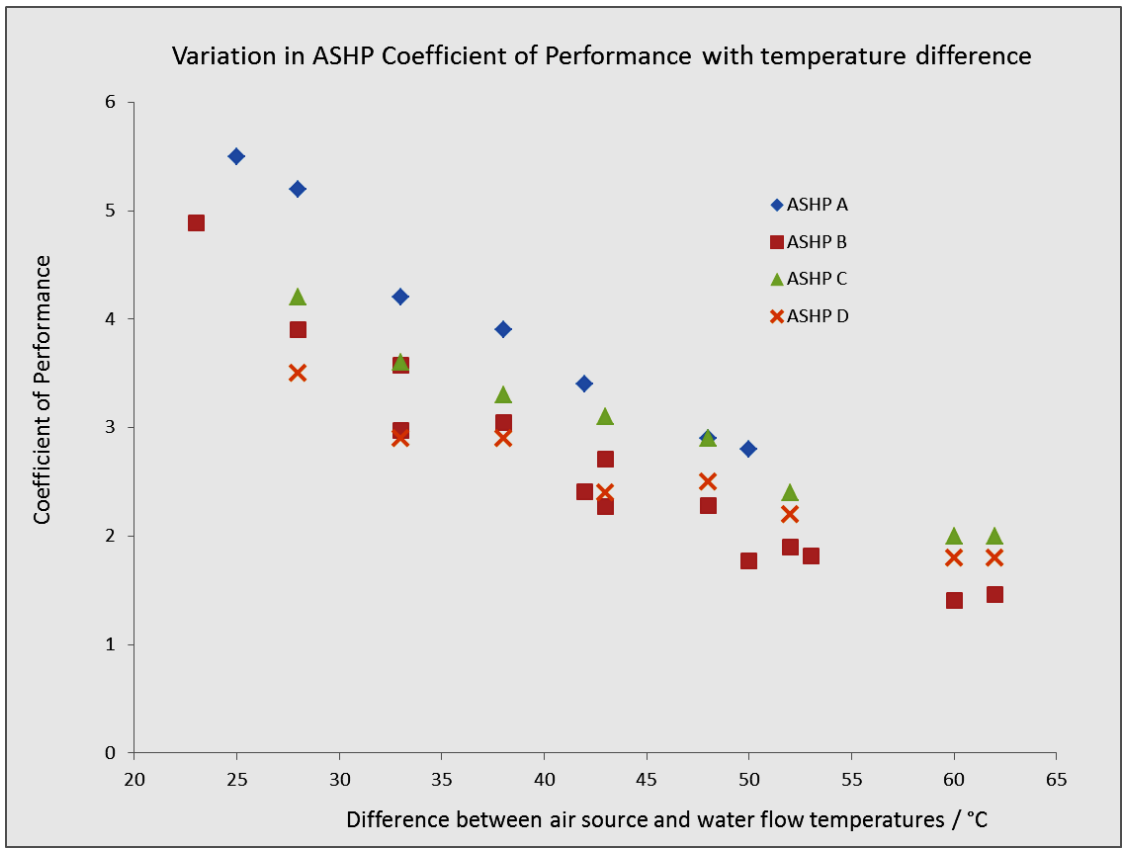
Figure 6: ASHP performance with variation in operating temperature. Data adapted from Butler & Hyde 2007; Warmepumpen-Testzentrum 2013; Energimyndigheten 2012.
