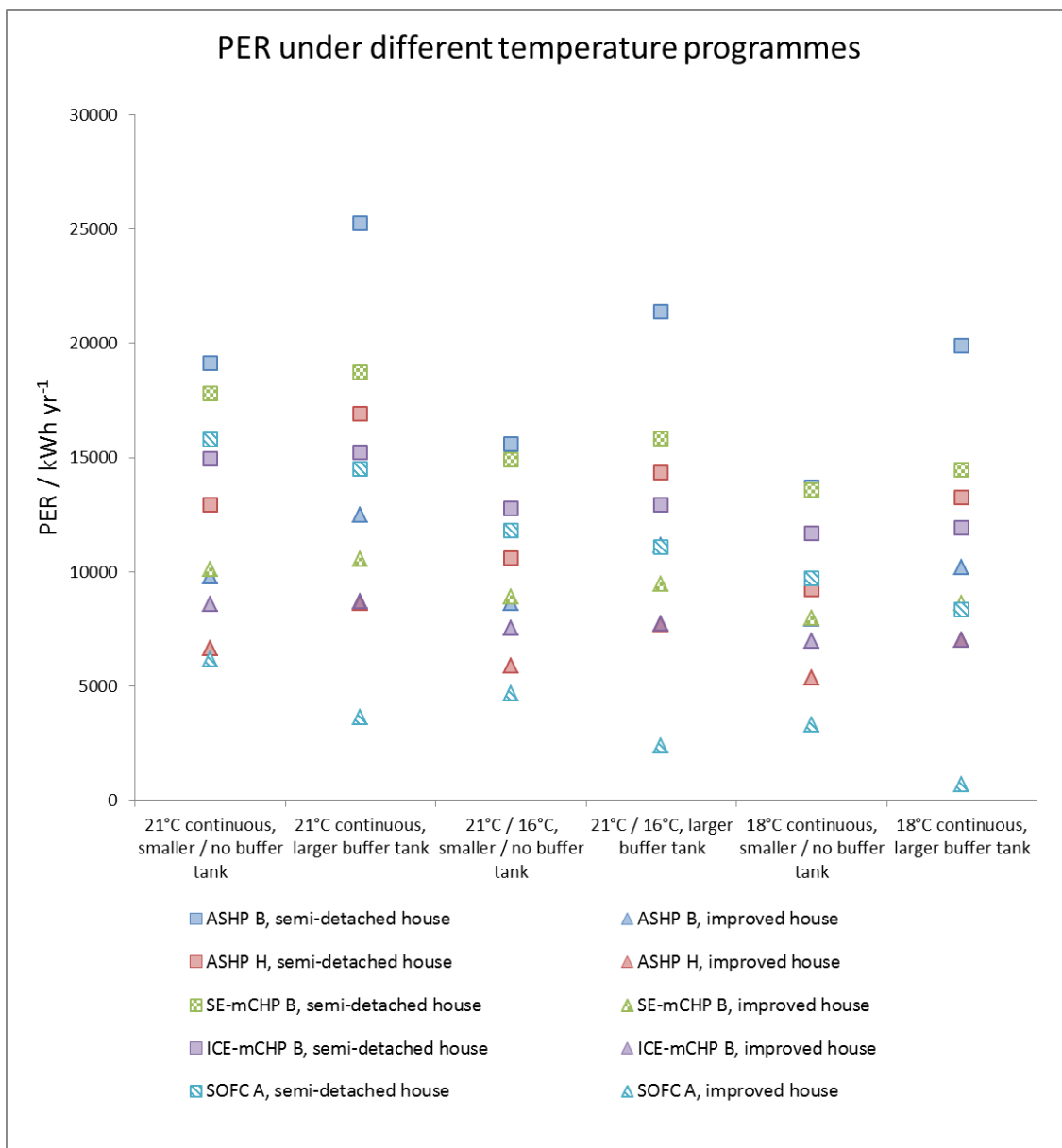
Figure 88: Effect of temperature programme on PER of selected units
