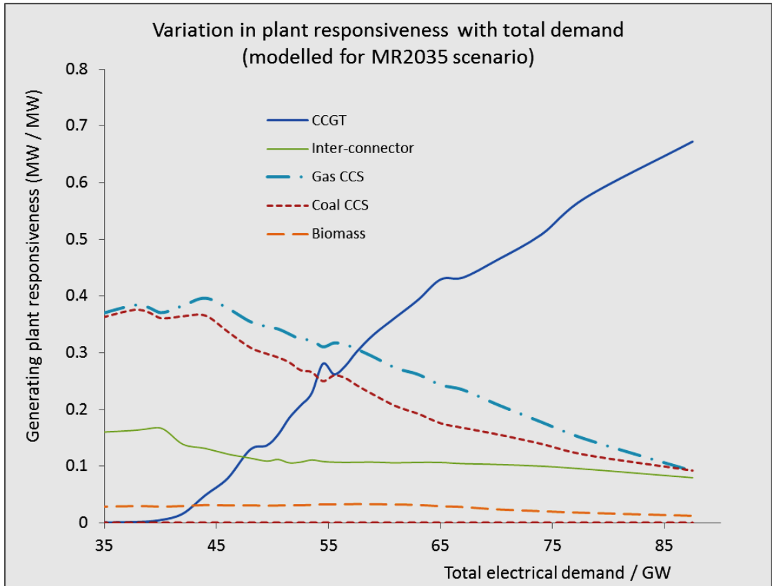
Figure 36: Variation in plant responsiveness with total demand (modelled for MR2035 scenario)
