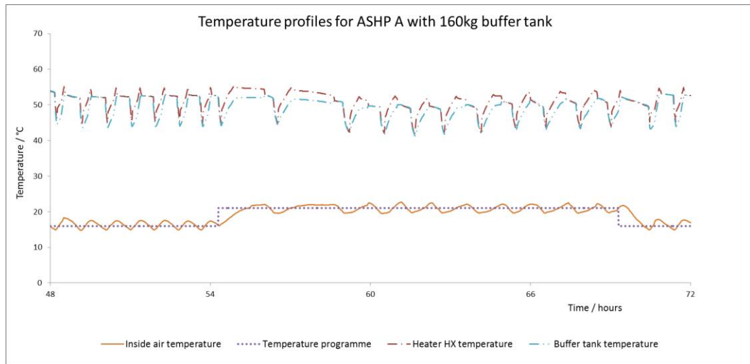
Figure 46: Example temperature profile with ASHP and buffer tank
