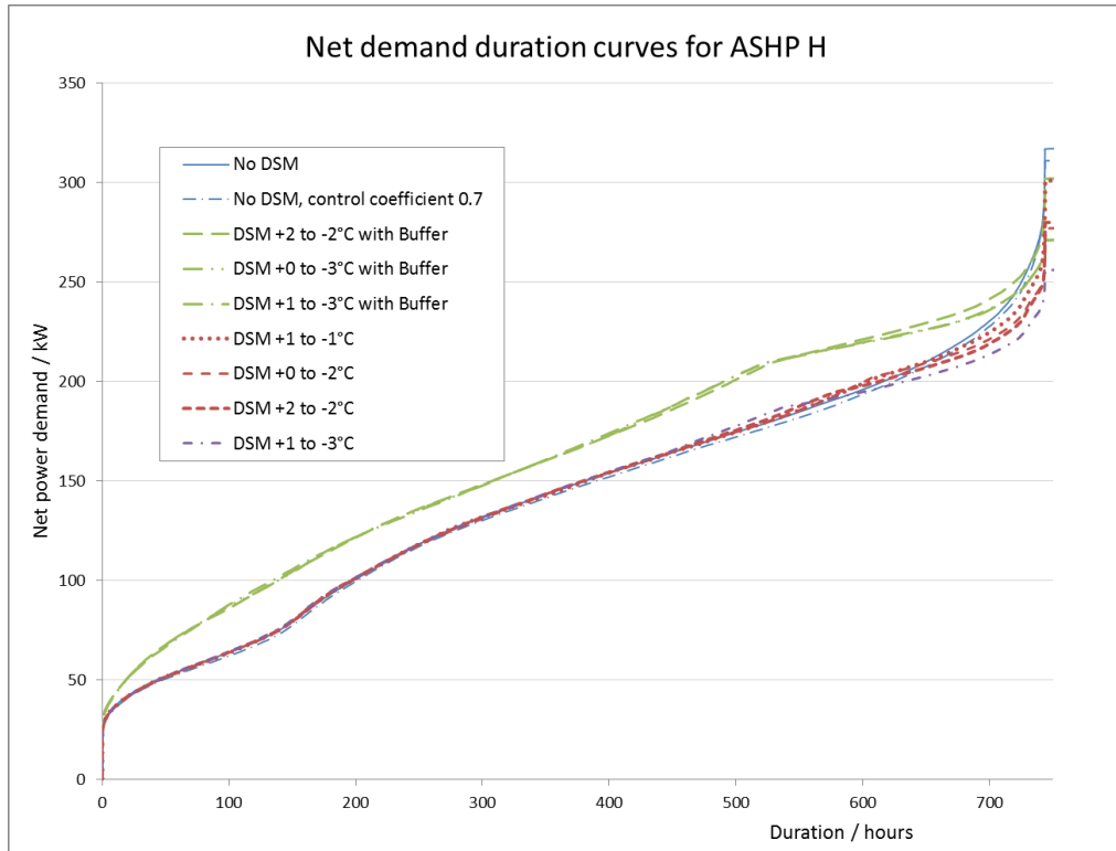
Figure 110: Net demand duration curves for neighbourhoods using ASHP H with DSM.
