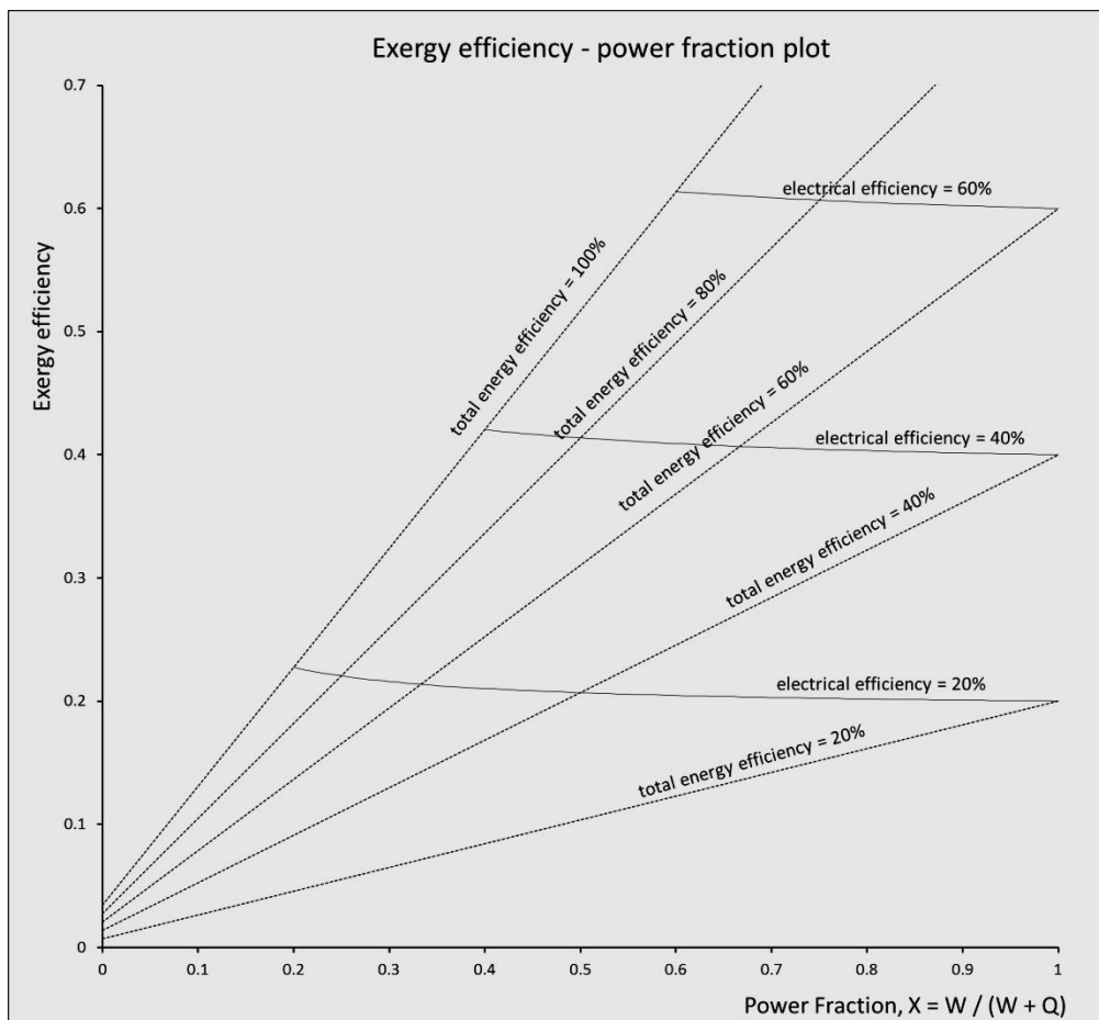
Figure 14: Effect on exergy efficiency of variation in power fraction
