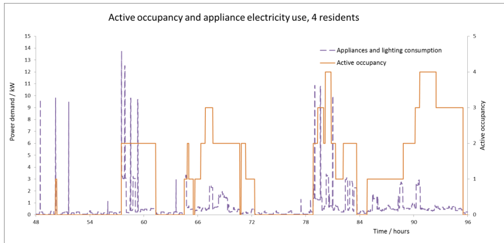
Figure 55: Example of active occupancy and appliance electrical demand for house with four residents
