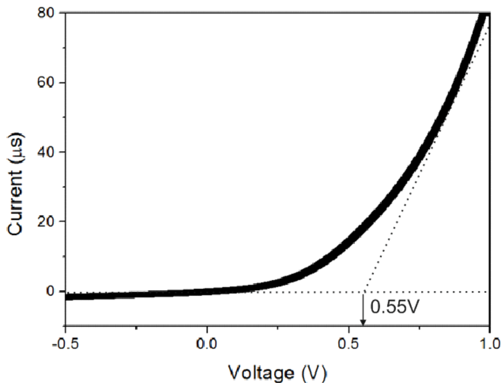
Figure 2.14 The I-V curve from the sixth p-n pair of sample A1.
