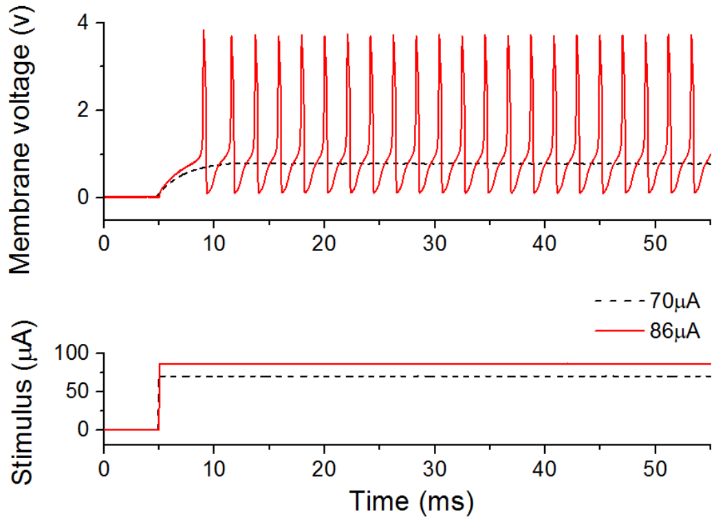
Figure 3.14 Response of a silicon neuron to direct current stimulus with different values. The trace represented by dash lines results from the stimulus of 70\mu\text{A} ; the trace represented by solid lines results from the stimulus of 86\mu\text{A} . Spikes arise only when the input current is above the threshold of 86\mu\text{A} . The amplitude of the spikes is 3.7\text{ V} .
