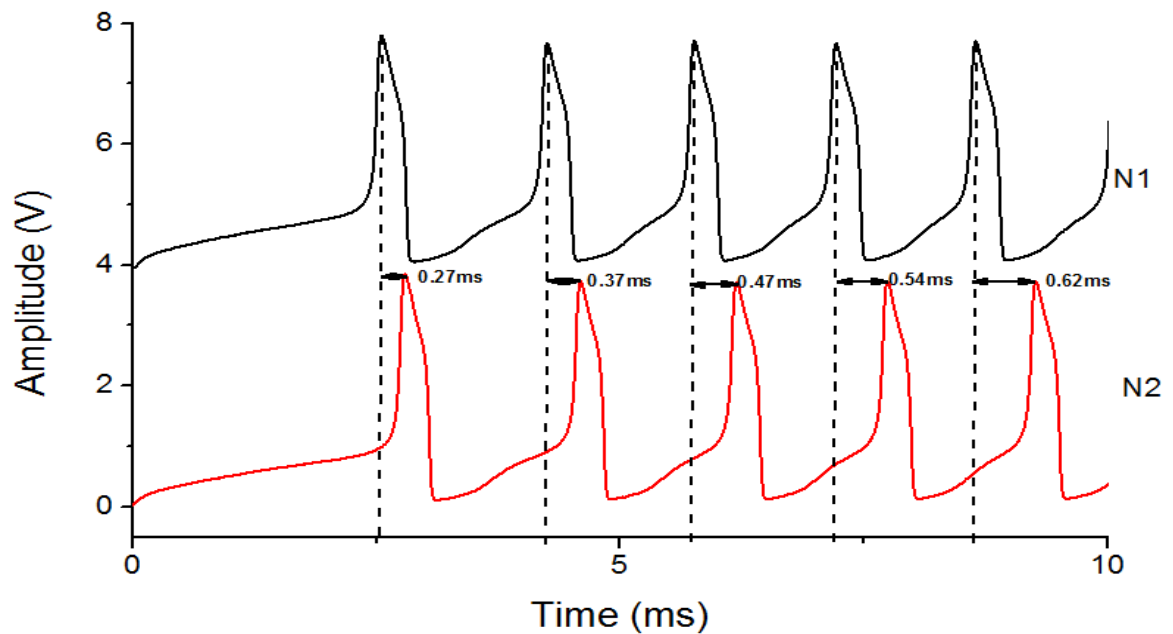
Figure 3.17 Firing sequence of two decoupled neurons. Each neuron is excited by a direct current of 100\mu\text{A} and oscillates at its own natural frequency. Time delays between spikes of the two neurons have been marked in the plot.
