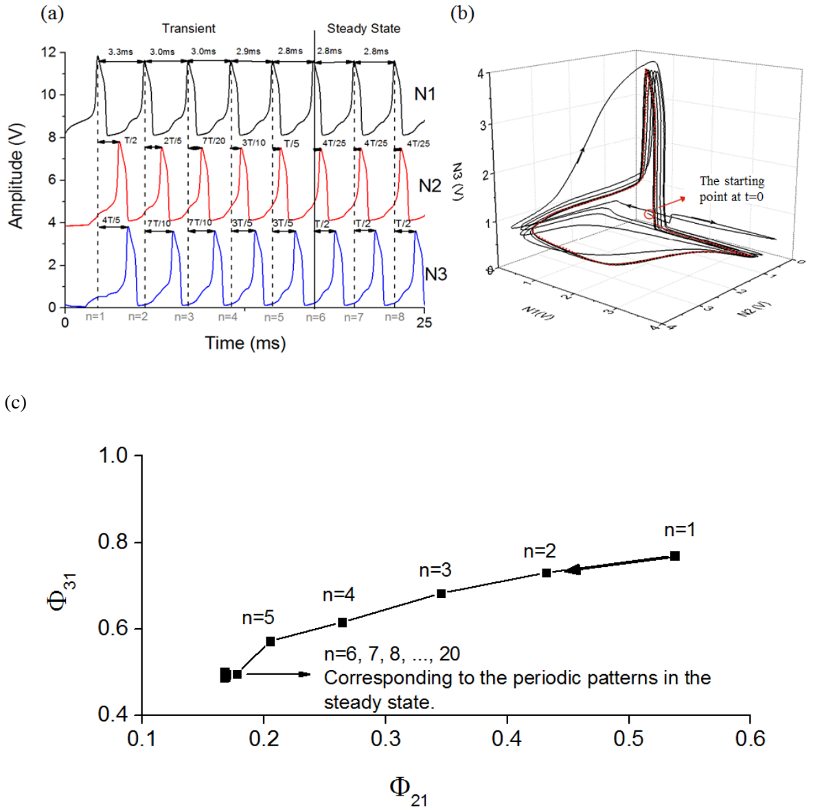
Figure 4.3 (a) Rhythmic patterns generated by the CPG when g_{12}=g_{23}=g_{31}=16 \mu\text{S} , g_{21}=g_{13}=g_{32}=45 \mu\text{S} . The magnitude of the stimulus current is 100 \mu\text{A} . The initial condition is (\Delta T_1=0.6, \Delta T_2=0.7) . The sequential activity of the neurons results from the competition without winner in the system. There is a transient region at the beginning in which the firing sequence is irregular. In the following steady region, the firing sequence is cyclic and periodic patterns are generated. (b) The three dimensional projection corresponding to the oscillations shown in (a). In the plot, each axis represents an oscillation voltage from one individual neuron. The steady patterns in (a) are shown as a limit cycle in this phase portrait. It is highlighted by a red dash line. The other part of the orbit that looks chaotic corresponds to the transient regime. (c) The forward trajectory of the firing sequence \{\Phi_{21}^n, \Phi_{31}^n\} ( n=1, 2, 3, \dots, 20 ). It is plotted according to the time delays shown in (a). N1-n5 indicates the transient time during which the time delays are varying. N6-n20 corresponds to the steady patterns which possess constant period and time delays. Spiking patterns in n9-n20 are not shown in (a) due to the limited space.
