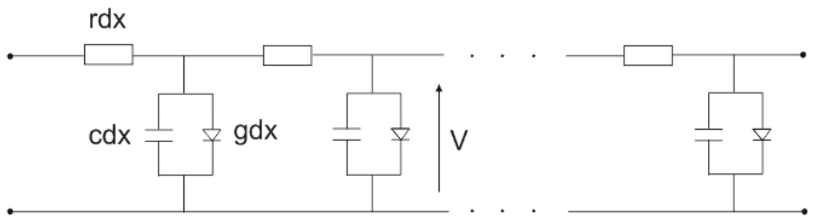
Figure 2.1 A transmission line circuit that represents the key electrical characteristics of the nerve fibre. In the circuit, the resistor mimics the axial resistivity of the capillary, the capacitor mimics the membrane capacitance, and the diode mimics the nonlinear conductance across the membrane [15].
