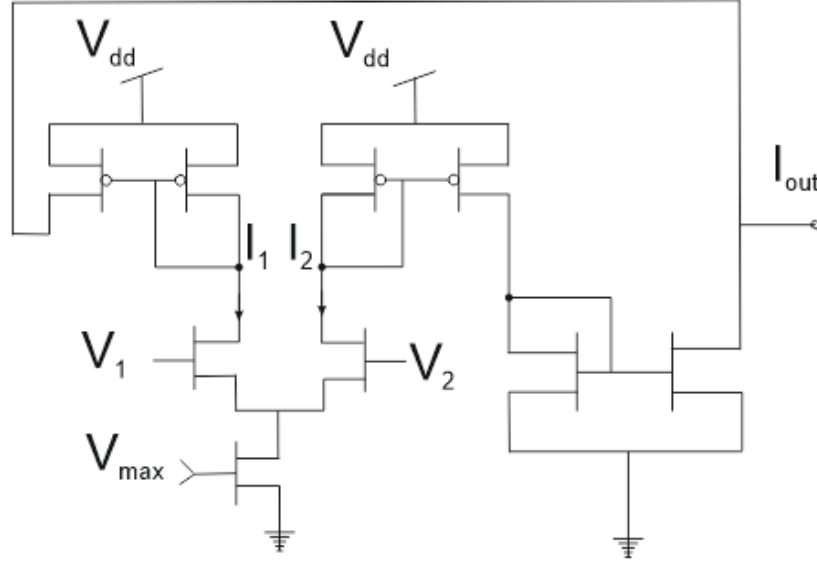
Figure 3.7 The circuit of an analogue gap junction synapse. V_1 and V_2 are the pre- and post-synaptic neuron membrane voltages. V_{max} determines the gain between I_{out} and (V_1 - V_2) .
