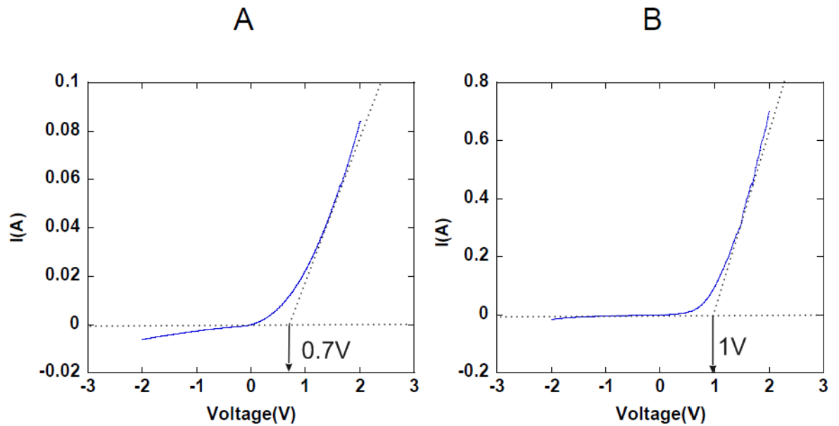
Figure 2.10 The I-V curves of p-n junction samples. They indicate the onset voltages of the junctions. The onset voltage of sample A is about 0.7V. And the onset voltage of sample B is about 1V.
