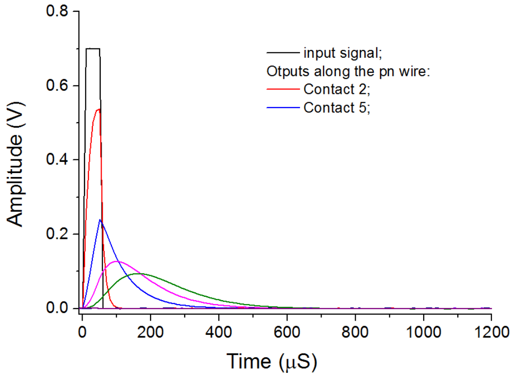
Figure 2.19 Pulse propagation along the transmission line when the magnetic field is tilted by 45 degrees to the normal.
