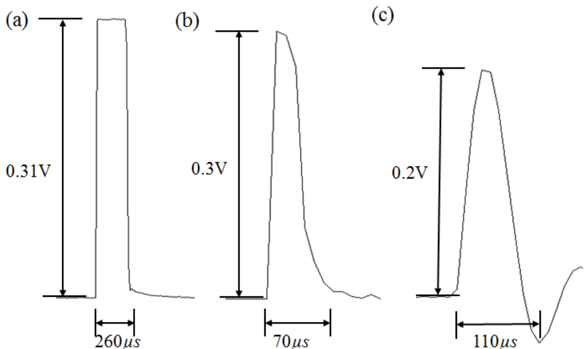
Figure 2.4 A plot to show the measured wave profiles of propagating waves created by input pulses with widths a) 250\mu\text{s} , b) 10\mu\text{s} and c) 5\mu\text{s} . The amplitude of the input pulse is 2\text{V} . All the measured wave profiles are all collected from node 1 of the transmission line shown in figure 2.3.
