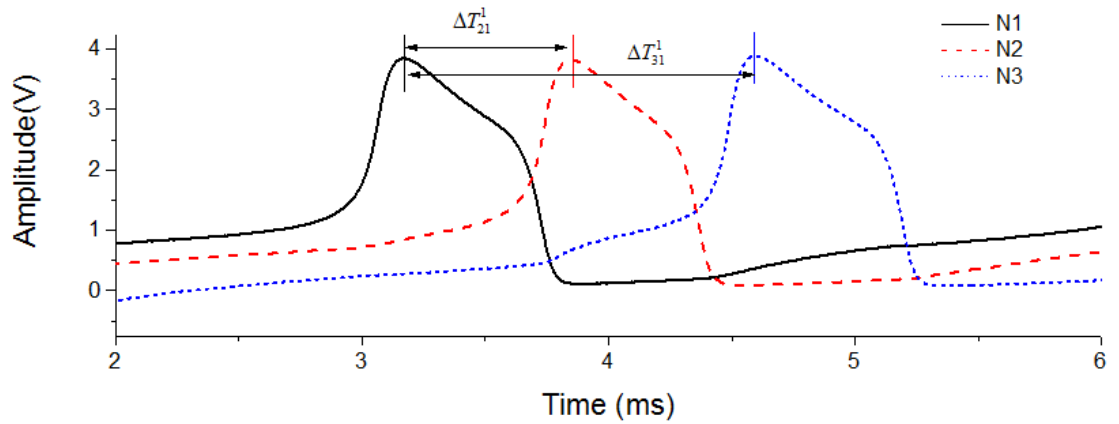
Figure 4.2 The time delay between the first peaks from different neurons. We use N1 as the reference neuron.
