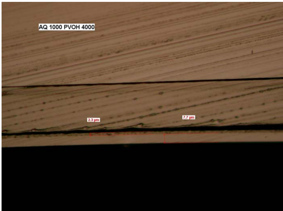
Figure 68: Cross section measurement of Aqualon N200 1000 rpm GH20 4000 rpm
