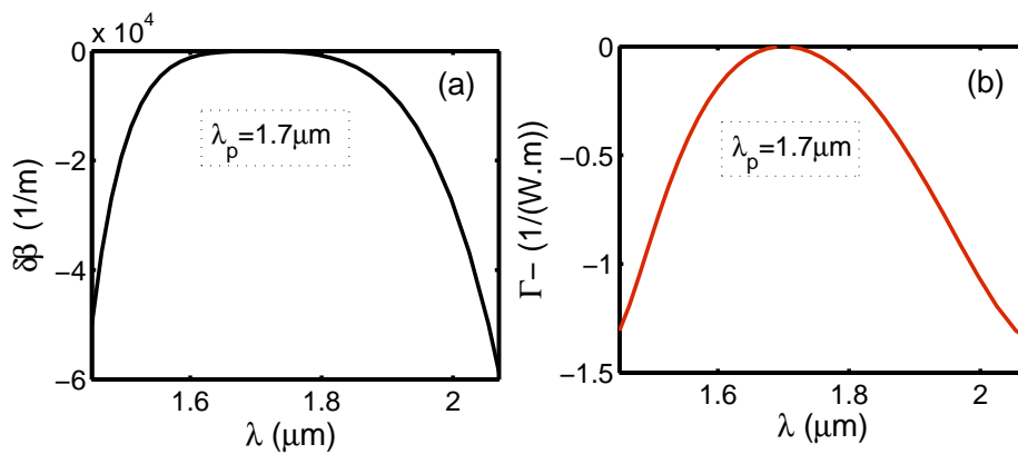
Figure 3.3.14: Plot of \delta\beta and \Gamma_- as function of signal and idler wavelengths for the slot waveguide. Geometry is same as Figure 3.3.13. D = -0.0003\text{ps/nm/mm} , n_{2,\text{glass}} = 3 \times 10^{-18}\text{m}^2/\text{W} , n_{2,\text{silicon}} = 4 \times 10^{-18}\text{m}^2/\text{W}
