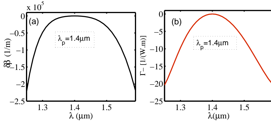
Figure 3.3.5: Plot of \delta\beta and \Gamma_- as function of signal and idler wavelengths at \lambda_p = 1.4 \mu\text{m} for 300\text{nm} \times 220\text{nm} SOI waveguide. n_2 = 4 \times 10^{-18} \text{m}^2/\text{W} , D = -2200 \text{ps}/\text{nm}/\text{Km} .
