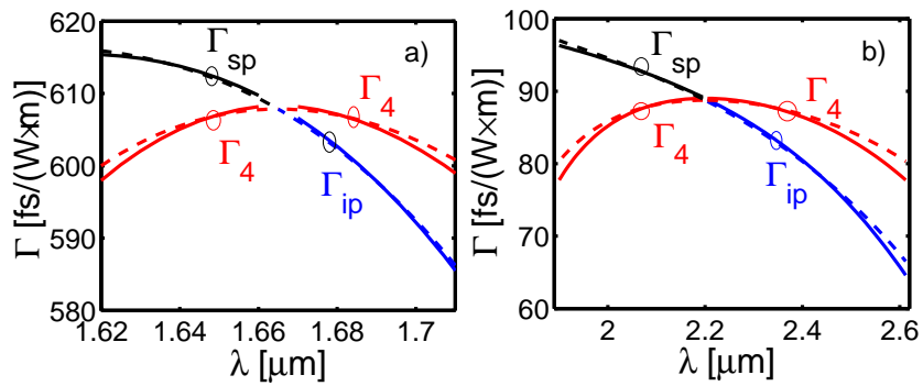
Figure 4.1.3: The plots of nonlinear coefficients \Gamma entering the necessary condition of MI [see equation 4.3.5] calculated for AlGaAs waveguide at \lambda_p = 1.665\mu m (a) and SOI waveguide at \lambda_p = 2.2\mu m (b). Dashed curves show their factorized approximations, see Equation 4.1.3.
