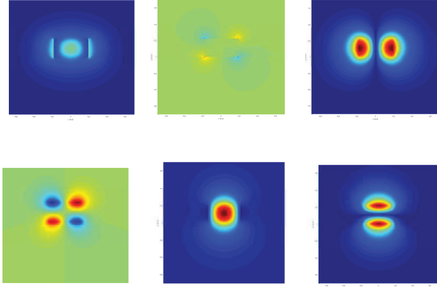
Figure 3.2.1: The profile of guided mode for 380nm \times 220nm SOI waveguide at pump wavelength \lambda_p=1.55\mu m . from left to right , in the first row, E_x , E_y , E_z . In the second row, H_x , H_y , H_z .
