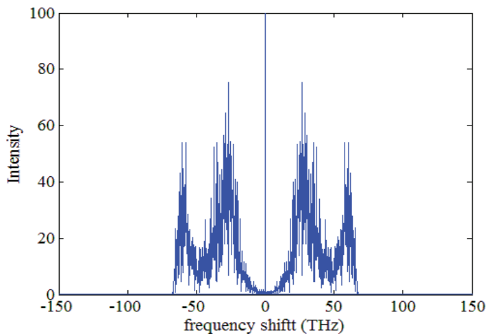
Figure 2.2.1: Spectral output of a 220\text{nm} \times 330\text{nm} silicon waveguide with initial power 1\text{W} and \lambda_p = 1.47\mu\text{m} . Spectral sidebands are due to modulation instability. (Note: this model doesn't include the TPA and free carrier effects.)
