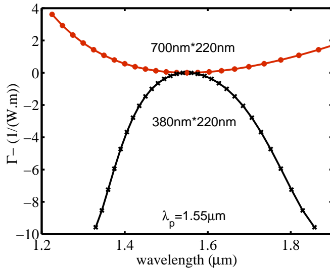
Figure 3.2.6: The plot of value of \Gamma_- as function of wavelength for 700\text{nm} \times 220\text{nm} (red curve with dot) and 380\text{nm} \times 220\text{nm} (black curve with cross) SOI waveguides. (Pump wavelength is 1.55\mu\text{m} for two cases.)
