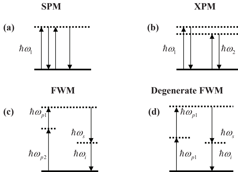
Figure 1.1.1: Schematic diagrams of possible energy level. Self-phase modulation (SPM), cross-phase modulation (XPM), degenerate and non-degenerate four-wave mixing (FWM).
