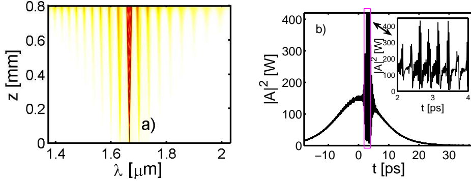
Figure 4.4.1: MI development with 10\text{ps} pulse excitation: (a) evolution of the spectrum with propagation distance and (b) output signal in time domain after the propagation distance of z = 0.8\text{mm} . The inset zooms in the central region of the pulse, where formation of a periodic sequence of ultra-short pulses is clearly visible. The pump/ seed peak power is 150\text{W}/0.1\text{mW} ; other parameters are the same as in Figure 4.3.4.
