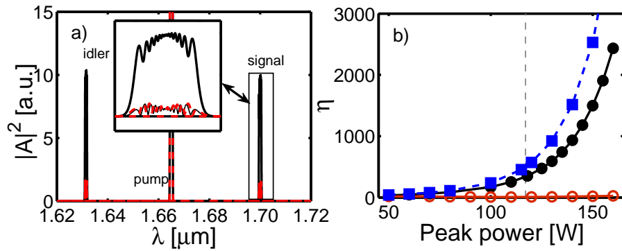
Figure 4.3.4: MI development with 100ps pulse excitation: (a) output spectra in frequency domain after z = 0.4mm propagation distance. The pump, signal and idler wavelengths are: \lambda_p = 1.665\mu m , \lambda_s = 1.7\mu m , \lambda_i = 1.6314\mu m . Thin solid curve corresponds to wavelength-independent nonlinearity, dotted red/gray curve to self-steepening only, and thick solid curve to full dispersion of nonlinearity. Pump peak power is 150W . The inset shows the MI at signal wavelength 1.7\mu m . (b) Conversion efficiency as a function of the pump peak power. Full/open circles correspond to the full/self-steepening only dispersion of nonlinearity. Full squares correspond to the same as full circles, but for 10ps pulse excitation. Vertical dashed line indicates the threshold power for the case of three interacting waves [126]. The signal peak power is fixed to 0.1mW in all simulations.
