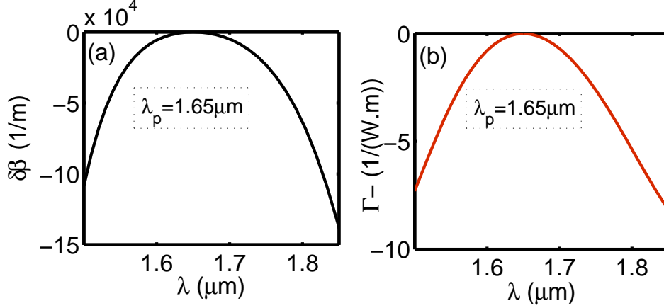
Figure 3.3.2: The plot of values of \delta\beta and \Gamma_- as functions of signal and idler wavelengths at \lambda_p = 1.65\mu\text{m} for 380\text{nm} \times 220\text{nm} SOI waveguide. n_2 = 4 \times 10^{-18}\text{m}^2/\text{W} , D = -3200\text{ps}/\text{nm}/\text{Km} .
