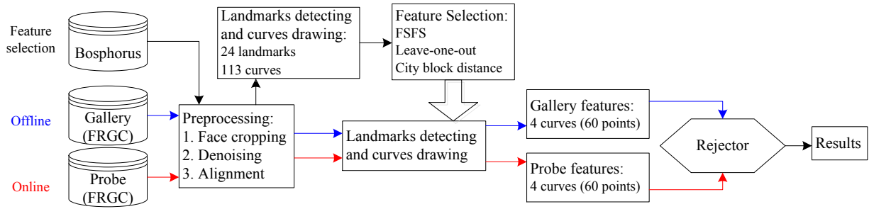
Figure 4.1: The block diagram of the proposed rejector.
