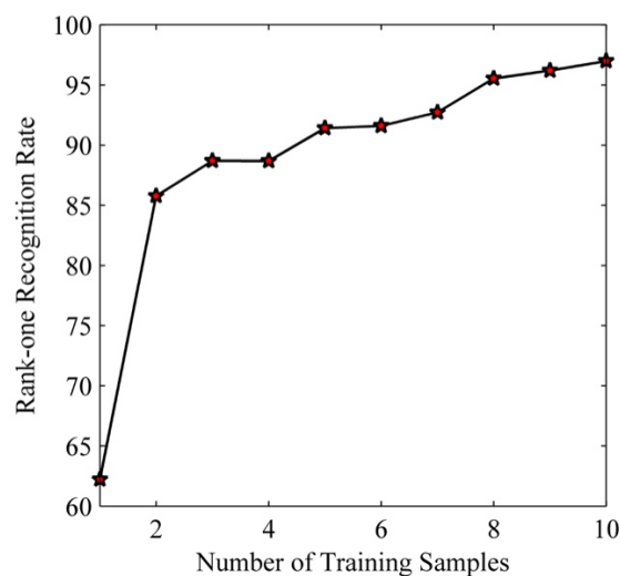
Figure 6.4: R_1RR s against the number of training samples using the selected curves from the SN_y map of the Photoface captures. All the captures in the Photoface database are used in this evaluation.
