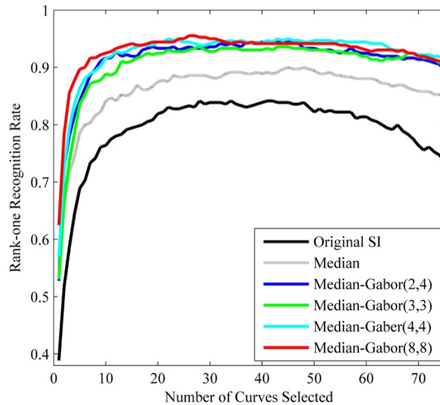
Figure 6.9: R_1RRs against the number of nasal curves selected for face recognition using the Gabor filters with different variances. For example, in Gabor (2,4), “2” and “4” are the variances along x and y axis, respectively. The frequency is set to “16”. 360 captures of 20 subjects from the Bosphorus database are used.
