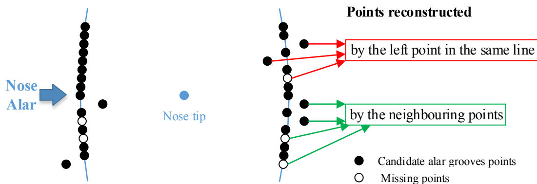
Figure 7.10: The diagram describes the missing points reconstruction and candidate alar grooves adjustment. For each missing or false detected point on the right alar, Dist_{right_i} , they are reconstructed on the basis of the pair on the same line. If the pair on the left is well detected, which is measured by T_c , the point on the right can be reconstructed directly by this pair and the location of nose tip. Otherwise, the point on the right should be interpolated by the neighbouring points.
