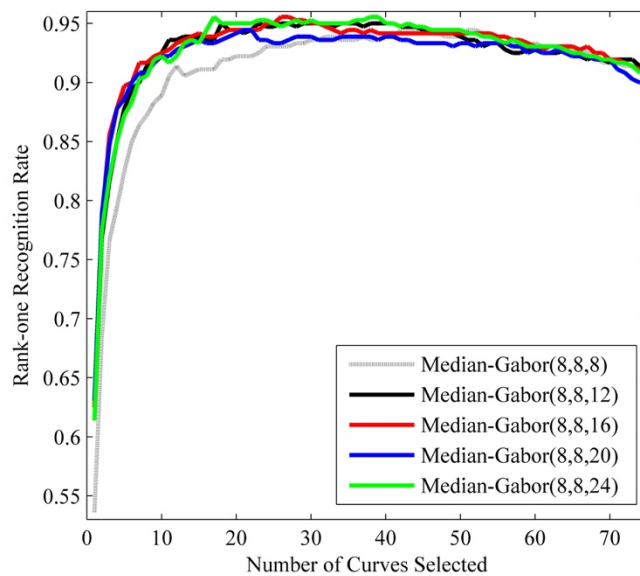
Figure 6.10: R_1RRs against the number of nasal curves selected for face recognition using the Gabor filters with different frequencies. For example, in Gabor (8,8,16), “8” and “8” are the variances and “16” is the frequency. 360 captures of 20 subjects from the Bosphorus database are used.
