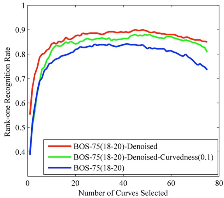
Figure 6.8: R_1RRs against the number of curves selected by FSFS using the capture selected from the Bosphorus database. It is a comparison of the recognition performance using the SI maps denoised by the median filter and curvedness thresholding.
