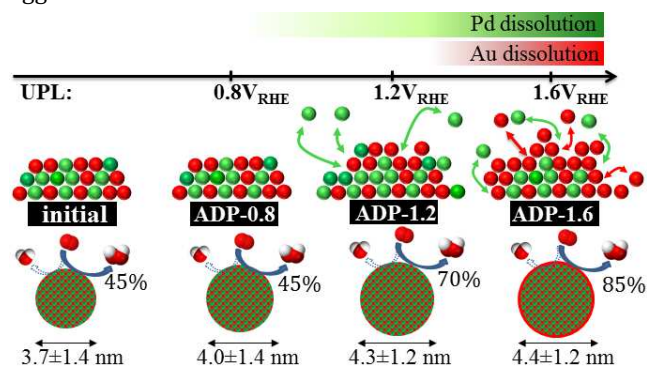
Scheme 1 Representative evolution of the surface composition and of the \text{H}_2\text{O}_2 selectivity (% values) during the ADPs.
