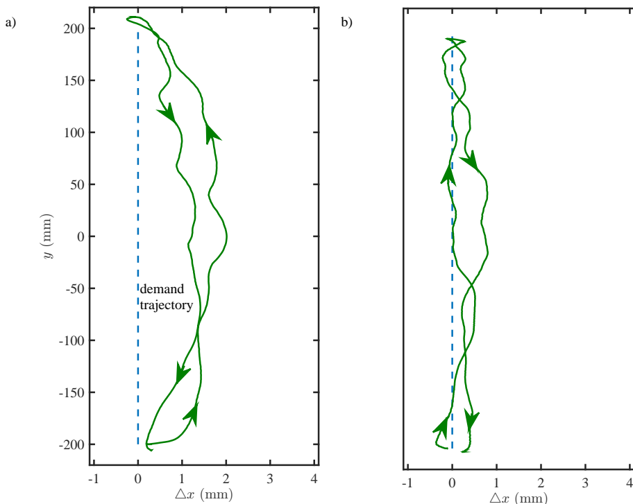
Figure 15. Measured linear trajectory control error \Delta x for a DR F with a) feedforward control derived using the flexure coupling model and b) implemented with a demand correction to minimise the displacement error.
