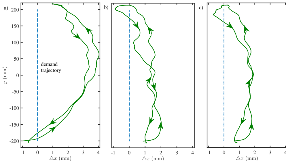
Figure 13. Experimental linear trajectory control error \Delta x for all joint types when feedforward control was derived using an idealised hinge assumption and implemented for a) DR_F , b) DR_L and c) DR_P .
