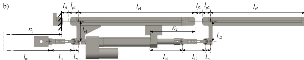
Figure 8. a) Experimental facility for double flexure coupling-rigid body system with components annotated and b) system parameters for mathematical model.
