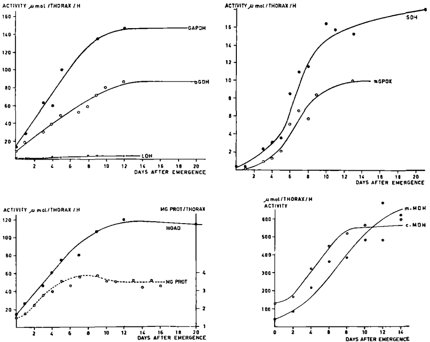
FIG. 2. The activities of different enzymes and the protein content per thorax as a function of time in the adult Colorado beetle reared under long-day conditions. Males were used throughout most of the experiments unless otherwise indicated. Each point reflects an average value derived from at least three determinations.
