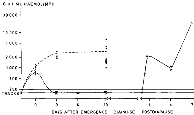
FIG. 8. Juvenile hormone titers (in Galleria units, G.U.) in the haemolymph of the adult Colorado beetle. Titers below 250 G.U. per ml of blood could not be evaluated quantitatively and are indicated as 'traces' After de Wilde et al (1968).
