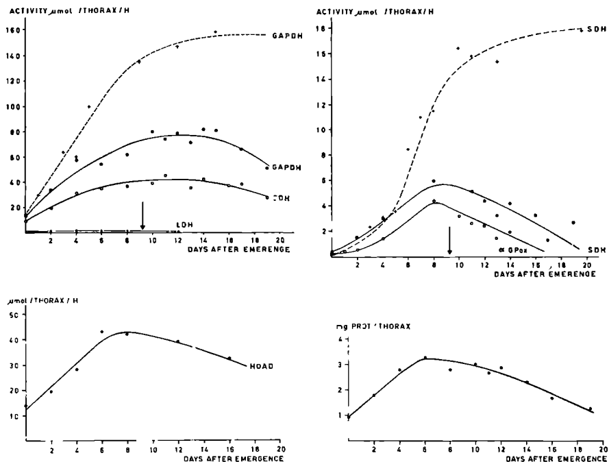
FIG. 6. The activities of different enzymes and the protein content per thorax in the adult Colorado beetle reared under short-day conditions.
