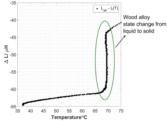
Figure 2. Measurements of the coil inductance differences versus the temperature changes during the solidification of a wood alloy.
